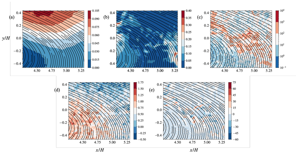
Figure 17: Instantaneous spatial distribution of (a) \tilde{k} , (b) k'k' , (c) \epsilon' , (d) \tilde{\omega} , and (e) \omega' with respect to the coherent vortex structure represented by solid line 2D streamlines in the case of SFV5 for G/H = 2.4 and Re = 1.0 \times 10^4 .
