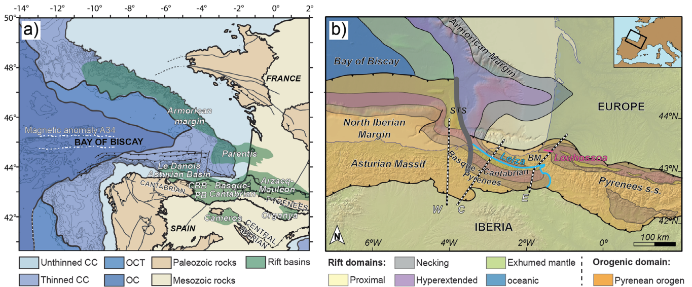
Fig. 2. (a) Map of the Mesozoic rift basins between France and Spain along the Iberian-European plate boundary. Modified after Lescoutre et al. (2021) and Masini et al. (2014) . (b) Rift domain map of the Pyrenean-Cantabrian area. STS: Santander Transfer System, W: Western section, C: Central section; E: Eastern section. Modified from Tugend et al. (2014) and Cadenas et al. (2020) . CC: continental crust; OC: oceanic crust; OCT: ocean-continent transition.
