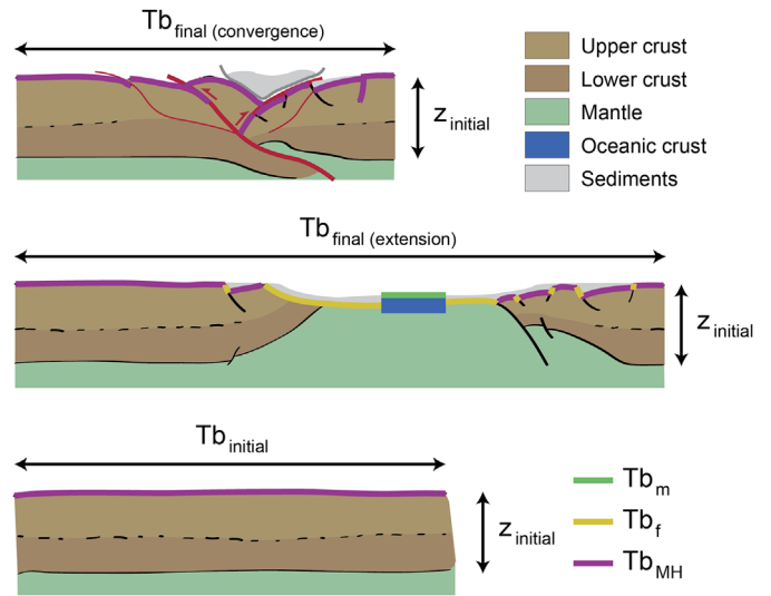
Fig. 5. Kinematic restoration of a crustal section back to the pre-rift stage with area conservation as well as pre-rift marker horizon length conservation (see text for further explanations). Tb: top basement; Tb m : magmatic top basement (new real estate); Tb f : fault top basement (new real estate); Tb MH : stratigraphic marker horizon top basement.
