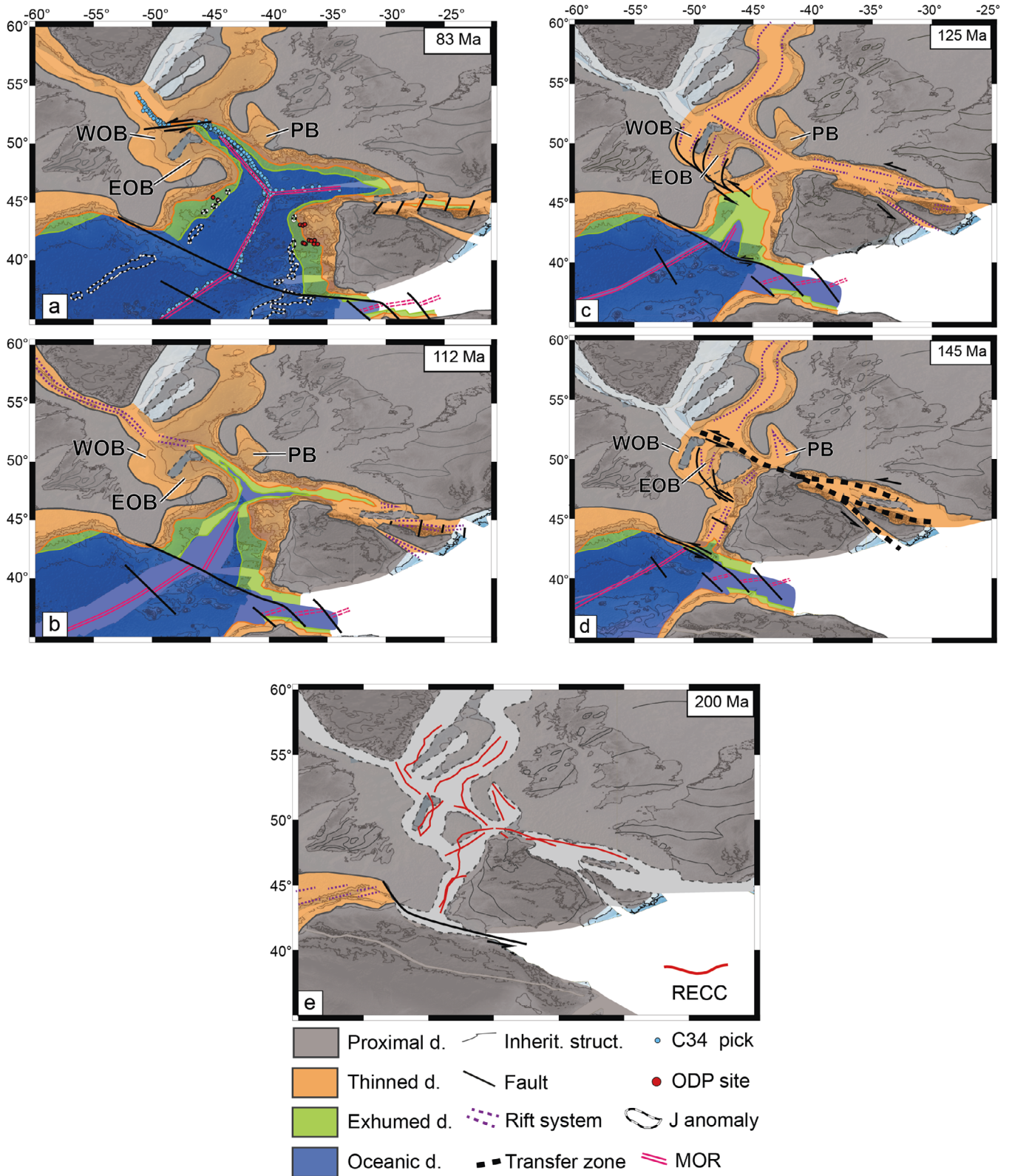
Fig. 4. Restoration of the southern North Atlantic, with North America fixed on present-day coordinates after Nirrengarten et al. (2018) with modifications for the Biscay Pyrenean domain based on Frasca et al. (2021) . (a) Santonian/Campanian (83 Ma), (b) Late Aptian/Albian (112 Ma), (c) Aptian (125 Ma), (d) Late Jurassic/Early Cretaceous (145 Ma), (e) end of Triassic (200 Ma). RECC: Reconstructed Edge of the Continental Crust. d.: domain; MOR: mid-oceanic ridge; EOB: East Orphan Basin; WOB: West Orphan Basin; PB: Porcupine Basin.
