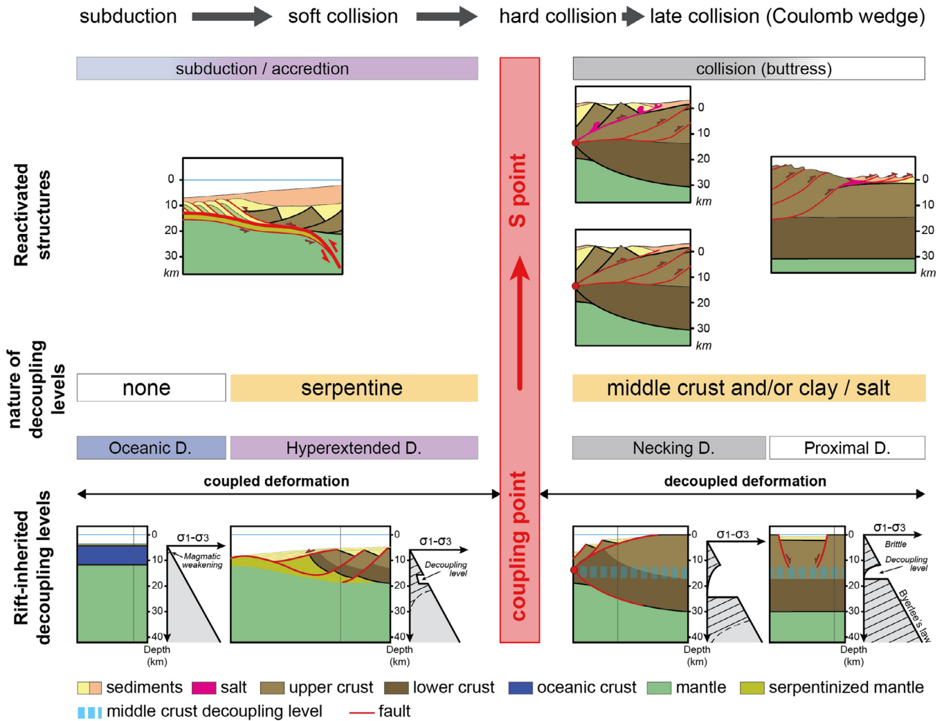
Fig. 10. Conceptual model illustrating the in-sequence reactivation of rift-inherited decoupling levels at a segment centre and explaining the transition from subduction to soft collision, to hard collision, and to final late collision (for details and discussion see text). Modified from Lescoutre and Manatschal (2020) and Miró et al. (2021).
