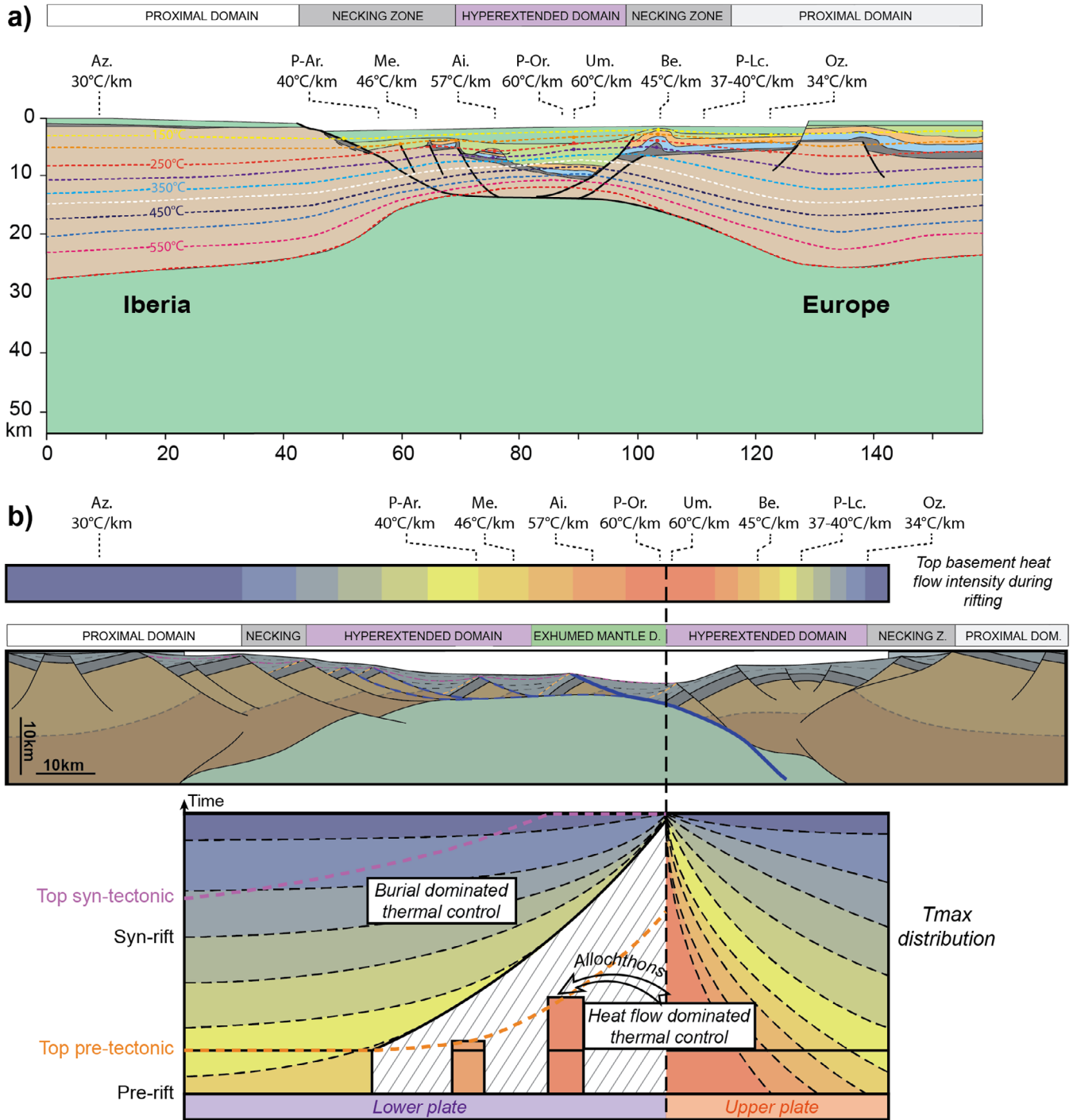
Fig. 8. Comparison of two published thermal models for the Mauléon basin: (a) the model from Saspiturry et al. (2020b) and (b) the model from Lescoutre et al. (2019) . The thermal gradients at the top of the two models are from Saspiturry et al. (2020b) (see text for details and discussion).
