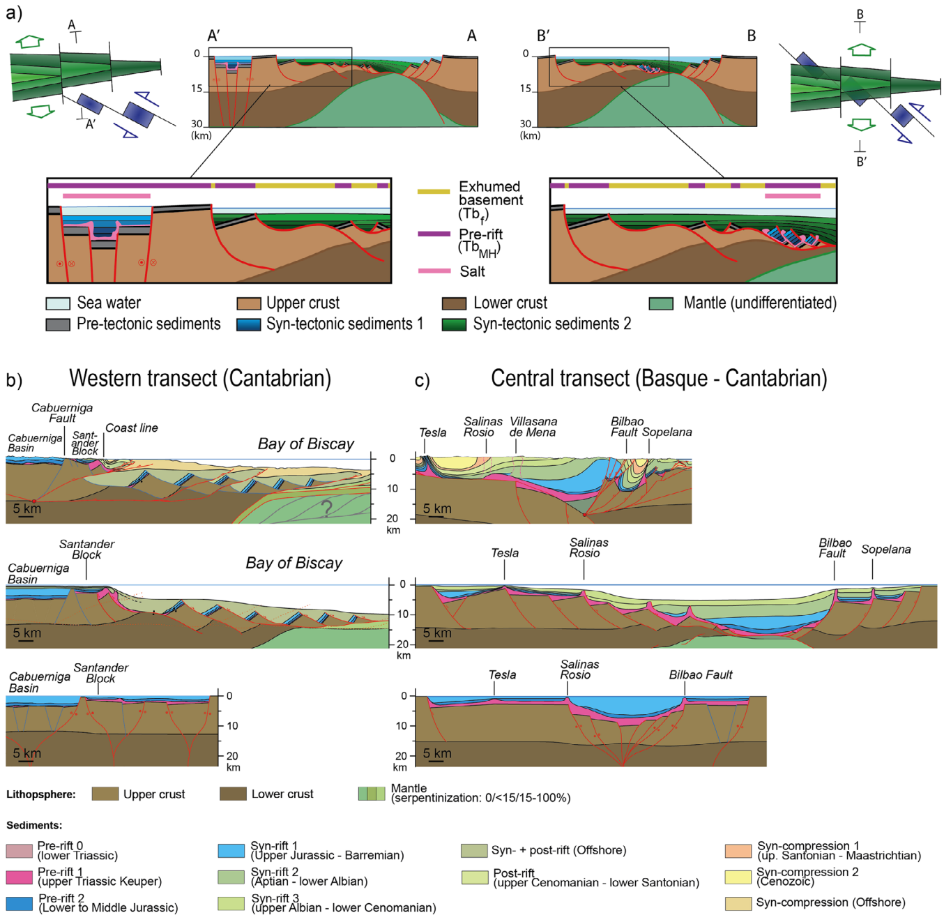
Fig. 7. (a) Schematic view of the two possible fates for Triassic (pre-hyperextension) salt in a multistage rift system: the top-left panel shows no interference/reactivation between salt bearing basins (blue) and subsequent hyperextended systems (green); the top-right panel shows full interference/overprint of salt bearing basins during later hyperextension (modified from Miró et al. , 2021 ). (b and c) Role of pre-rift salt during rifting and Alpine reactivation in the Asturias (b) and Basque-Cantabrian (c) transects (from Miró et al. , 2021 ); Note that these sections are zooms on the sections displayed in Figure 6 .
