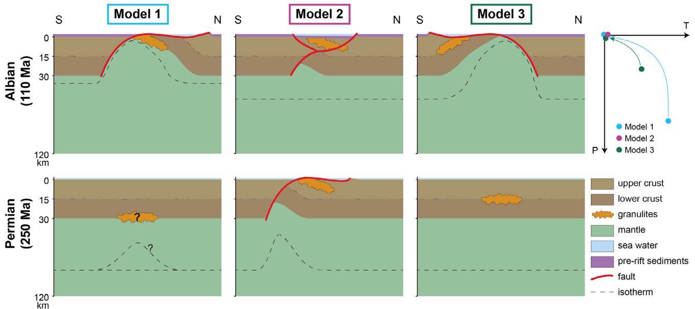
Fig. 9. Three competing models to explain the “granulite conundrum” in the Biscay-Pyrenean domain. See text for a more detailed description of the models and their implications.
