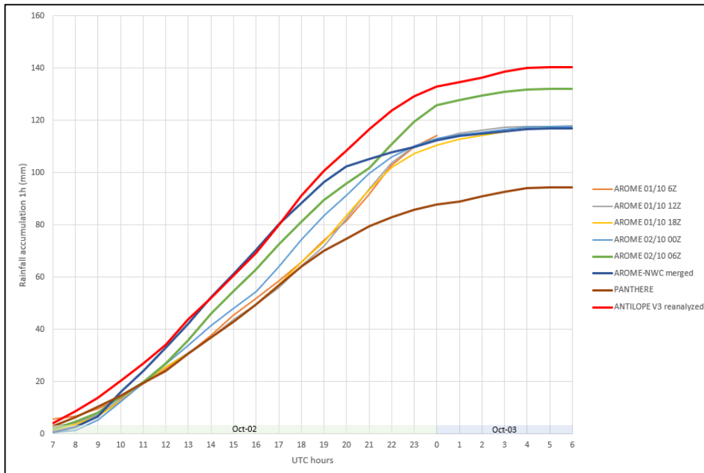
Figure 16: Accumulated hourly precipitations over the ROI (defined in Figure 14 ) for ANTILOPE-reanalyzed (red line), PANTHERE (brown line), AROME-NWC (dark blue), and several runs of AROME-FR
