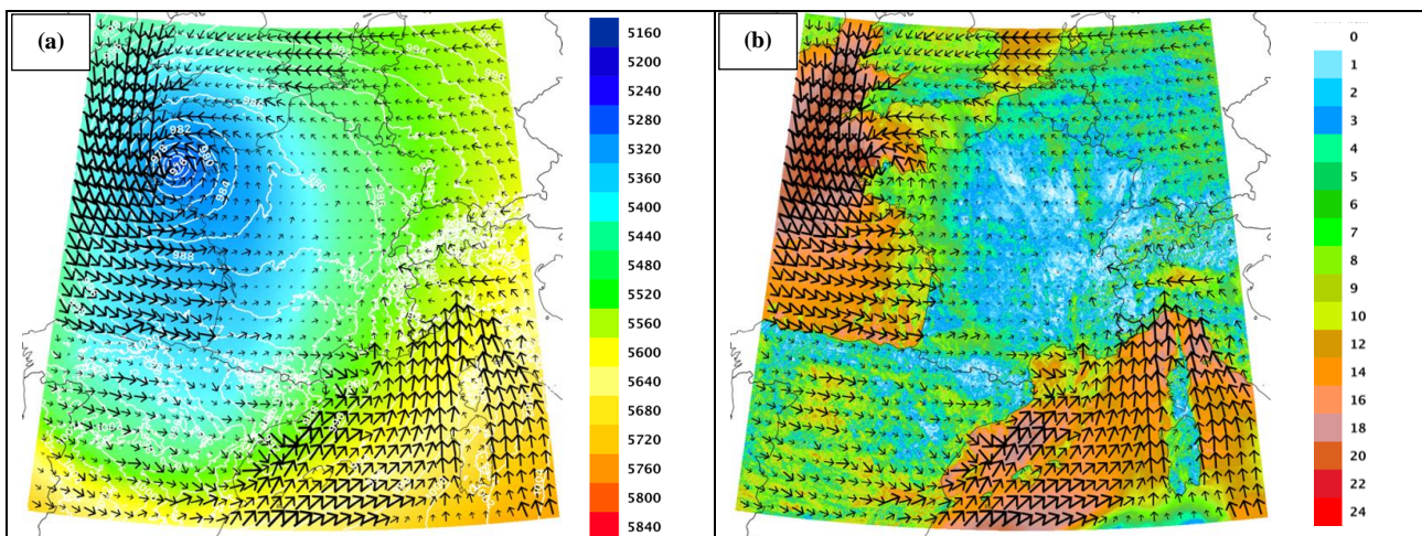
Figure 5 : Synoptic situation on October 2 nd 2020 6h UT modeled by AROME 2.5km resolution : (a) Geopotential height 500 hPa (m), surface and flow pressure (hPa) ; (b) Wind speed (m/s) and direction at 1000 hPa
