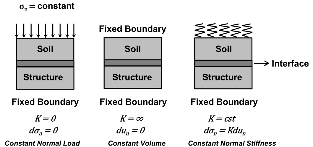
Figure 20. Boundary conditions of interface shearing (after Pra-ai [12]).
