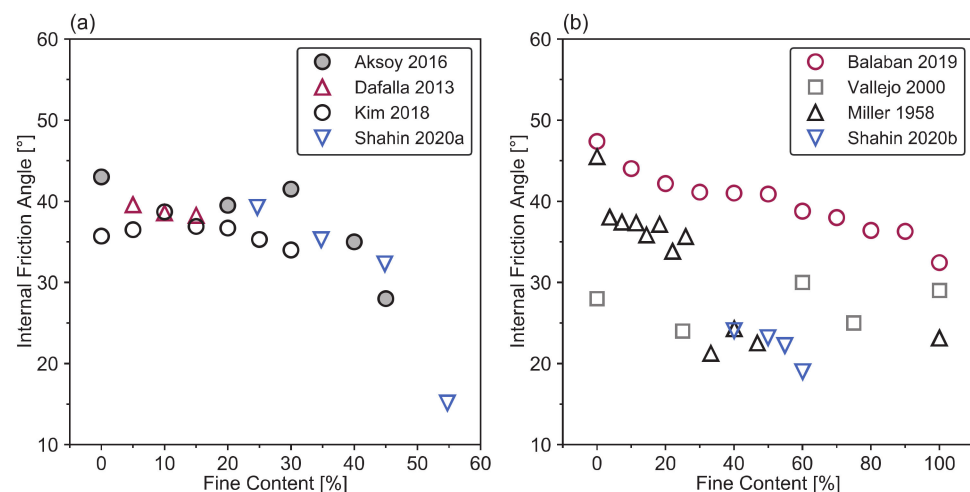
Figure 7. (a) and (b): internal friction angles of the sand–fines mixture as a function of fines content from the literature.
