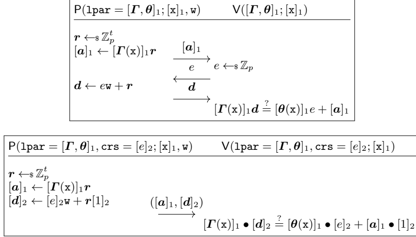
Fig. 8. The CHM \Sigma -protocol for algebraic languages \mathcal{L}_{\boldsymbol{\Gamma}, \boldsymbol{\theta}} (above) and its Couteau-Hartmann compilation \Pi_{\Sigma}^{\mathcal{C}} (below)
