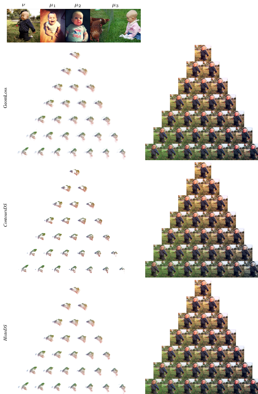
Figure 15: Color grading obtained by transferring the colors of n = 3 images onto a target image, aiming at reproducing with our method the results from (Bonneel et al., 2015), figure 12. Results are shown in triangles (Left: interpolated chrominance histograms; Right: corresponding transfer results). The images corresponding to the target chrominance histogram \nu and to the histograms \mu_i - which are interpolated to obtain a barycenter - are shown in top row. Each \mu_i corresponds to a vertex of the triangle in a clockwise order beginning with i = 1 at the uppermost vertex. Each row presents the results for a different method, from top to bottom: GeomLoss, our model trained on synthetic shape contours ( ContoursDS ) and our model trained on chrominance histograms from Flickr images ( HistoDS )
