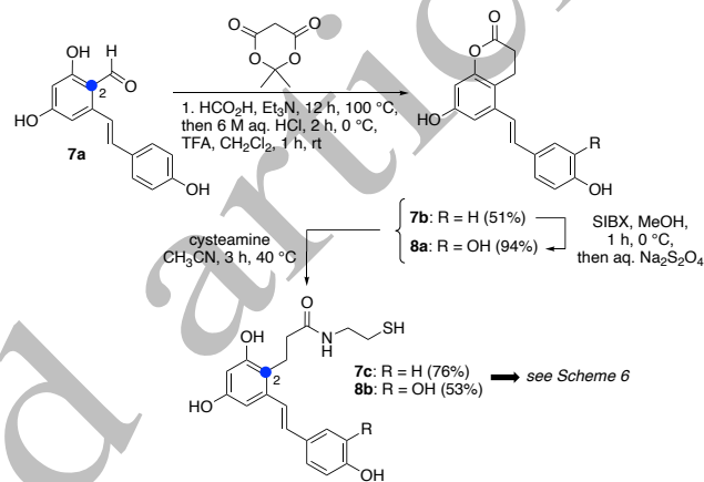
Scheme 5. Synthesis of resveratrol- and piceatannol-C2-propanamido sulfhydryl derivatives 7c and 8b .
