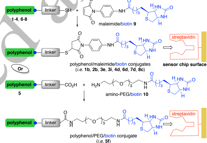
Figure 2. Schematic illustrations of the design and synthesis of polyphenol-biotin conjugates and their binding to streptavidin-coated sensor chips.
