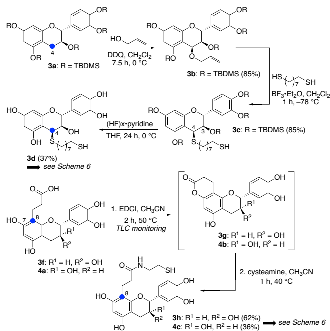
Scheme 2. Synthesis of the catechin-C4-thioether sulfhydryl derivative 3d and of the catechin- and epicatechin-C8-propanamido sulfhydryl derivatives 3h and 4c .
