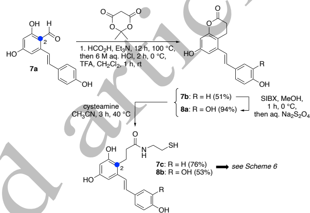
Scheme 5. Synthesis of resveratrol- and piceatannol-C2-propanamido sulfhydryl derivatives 7c and 8b .
