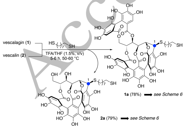
Scheme 1. Synthesis of the C1-deoxy vescalagin- and vescalin-C1-thioether sulfhydryl derivatives 1a and 2a . [2e,8a]
