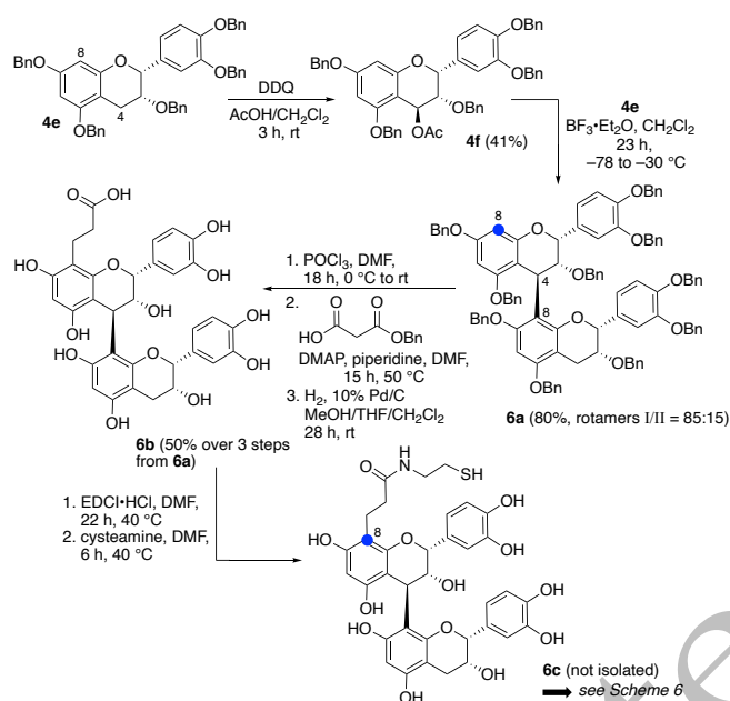
Scheme 4. Synthesis of the procyanidin B2-C8-propanamido sulfhydryl derivative 6c .
