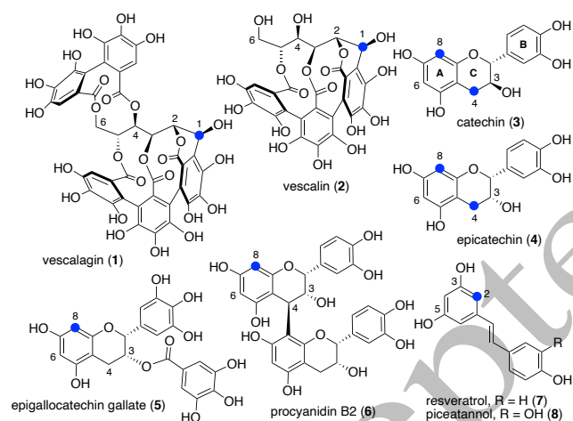
Figure 1. Selected plant polyphenols of different representative structural classes. Blue dots indicate the carbon sites of attachment of biotin-terminated units linked to these polyphenolic molecules.
