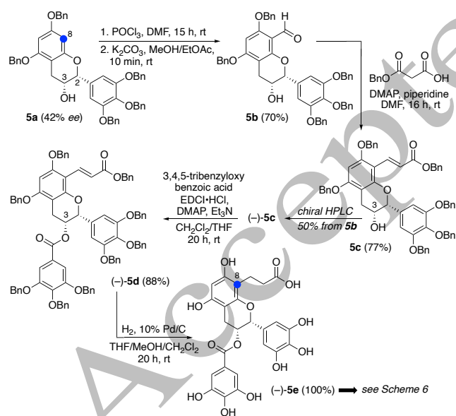
Scheme 3. Synthesis of the epigallocatechin gallate-C8-propanoic acid derivative 5e .
