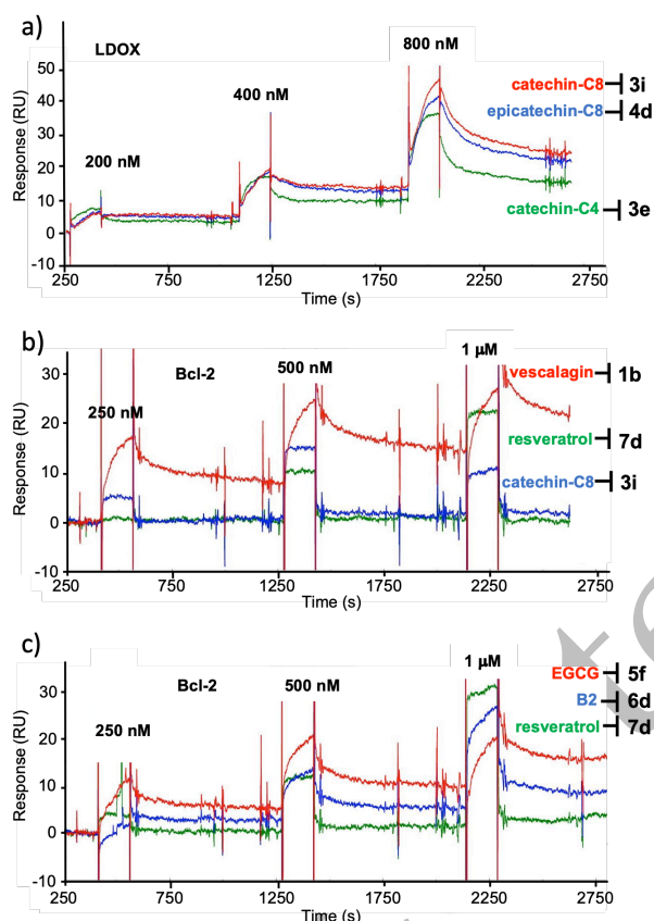
Figure 5. (a) Chip-B sensorgrams recorded upon injections of LDOX at 200-800 nM concentrations; (b) Chip-C and (c) chip-D sensorgrams recorded upon injections of Bcl-2 at 250-1000 nM concentrations.
