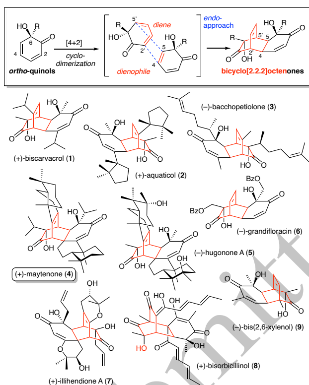
Figure 1. Examples of natural Diels–Alder cyclodimers of ortho -quinols. All of these natural products of plant or microbial origins are elaborated by a [4+2] cyclodimerization of ortho -quinols that strictly follows the same rules of site-specific regioselectivity and stereoselectivity. R = alkyl groups.
