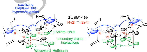
Figure 4. Cyclodimerization of the ferruginol-derived ortho -quinol into (+)-maytenone ( 4 ). This simplified drawing of the C_2 -symmetric Diels–Alder TS-A (the terpenoid decalin motif connected at C3 and C4 of the ortho -quinol monomer (6 R )- 18b is omitted for clarity) shows the positioning of the
