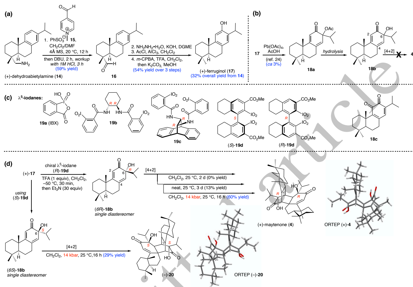
Figure 2. Chemical synthesis of (+)-maytenone ( 4 ) and its diastereomer (-)- 20 : (a) Preparation of (+)-ferruginol ( 17 ) from (+)-dehydroabietylamine ( 14 ). [26] (b) Johnson's early attempts to generate 4 from 17 through a dearomative oxygenation/[4+2] cycloaddition sequence. [24] (c) Structures of \lambda^5 -iodanes 19a-d used as oxygen-atom transfer reagents for the dearomative oxygenation of 17 , and structure of 8,12-abietadiene-11,12-dione ( 18c ), the undesired ortho -quinone resulting from the use of the \lambda^5 -iodanes 19a-c . (d) The completion of our 6-step asymmetric synthesis of (+)- 4 and its diastereomer (-)- 20 through the regio- and diastereoselective dearomative oxygenation of (+)- 17 by using the biphenylic \lambda^5 -iodanes (R)- 19d or (S)- 19d , respectively, followed by the site-specific regio- and diastereoselective [4+2] cyclodimerization of the ortho -quinols (6R)- 18b or (6R)- 18b under high pressure conditions.
