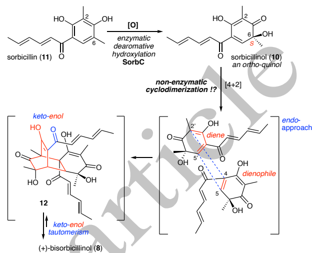
Scheme 1. Final steps of the biosynthesis of (+)-bisorbicillinol ( 8 ). This polyketide metabolite derives from the [4+2] cyclodimerization of the ( S )-enantiomer of sorbicillinol ( 10 ), the access to which being stereocontrolled by the enzyme SorbC that mediates the enantioselective dearomative hydroxylation of sorbicillin ( 11 ).
