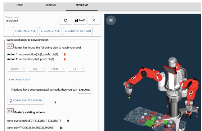
Fig. 9 The iRoPro interface showing the problems menu and the action sequence generated by the task planner.
