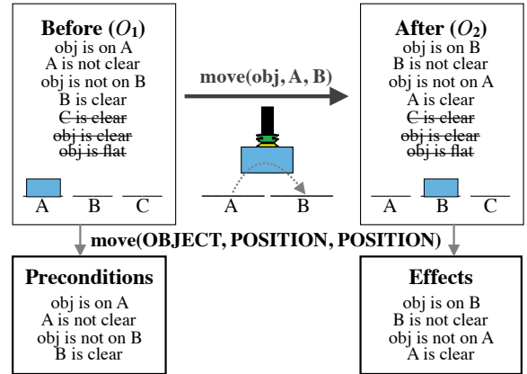
Fig. 7 Example of a high-level action for moving an object from A to B. Conditions are inferred from the observed predicates before ( O_1 ) and after ( O_2 ) the demonstration [28].
