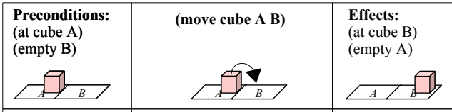
Fig. 2 Action model representation to move a cube from position A to B in terms of preconditions and effects [26].
