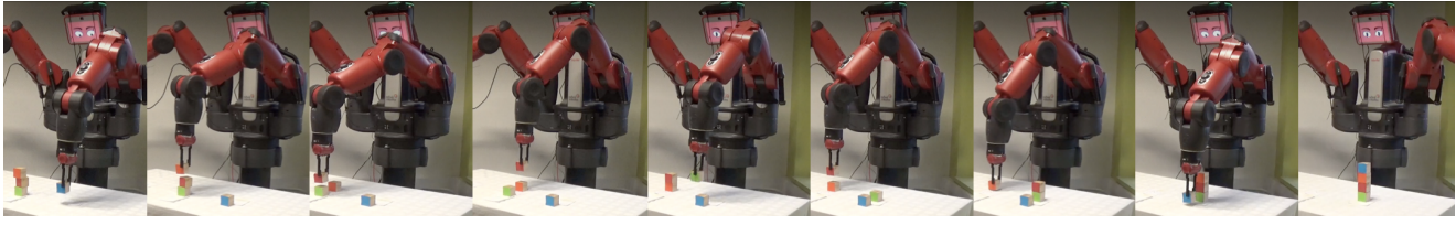
Fig. 12 Snapshots of an example task execution for stacking CUBE objects with the claw gripper.
