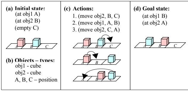
Fig. 1 Definition of a planning problem (a) properties describing the initial world state (b) object names and their types (c) instantiated actions (d) properties describing the goal [26].
