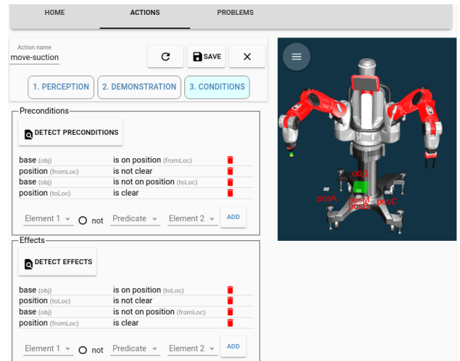
Fig. 8 The iRoPro interface showing the action condition menu and an interactive visualisation of the Baxter robot and detected objects.
