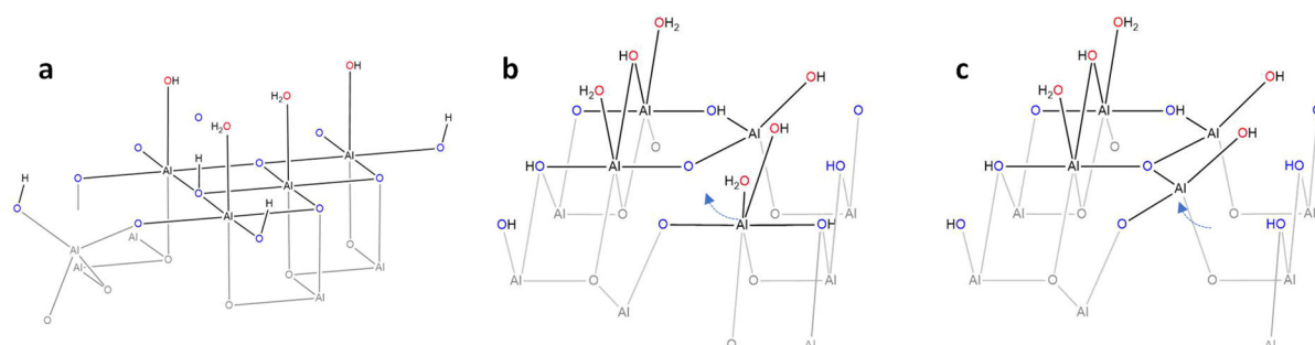
Figure 3: Schematic perspective view of the hydrated \gamma\text{-Al}_2\text{O}_3 reference surface structures. Oxygen atoms originating from water adsorbed molecules are shown in red, the ones from the bulk \gamma\text{-Al}_2\text{O}_3 are shown in blue. Surface aluminum atoms are shown in black, the subsurface ones in grey. (a) (1 0 0) facet has 4 inequivalent octahedral \text{Al}_{\text{VI}} exposed for adsorption, which can accept one \text{H}_2\text{O} molecule each; (b) the n(1 1 0) facet exposes 3 inequivalent octahedral \text{Al}_{\text{VI}} and 1 tetrahedral \text{Al}_{\text{IV}} site: \text{Al}_{\text{IV}} binds one \mu_1 -OH, the two neighboring \text{Al}_{\text{VI}} bind to \mu_1 -OH, \mu_1 -OH 2 and \mu_2 -OH and the further \text{Al}_{\text{VI}} presents two adsorption sites and binds to \mu_1 -OH and \mu_1 -OH 2 ; (c) the reconstructed R(1 1 0) facet results from the migration of one \text{Al}_{\text{VI}} to an \text{Al}_{\text{IV}} site (represented by the arrows), which induces the loss of one chemisorbed water, the transformation of a \mu_3 -OH into a \mu_2 -OH, and some proton rearrangements.
