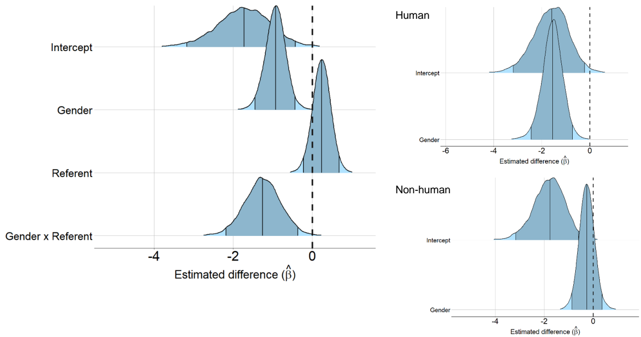
Fig.12. Posterior distributions of parameters for pronoun choice in Experiment 4.
