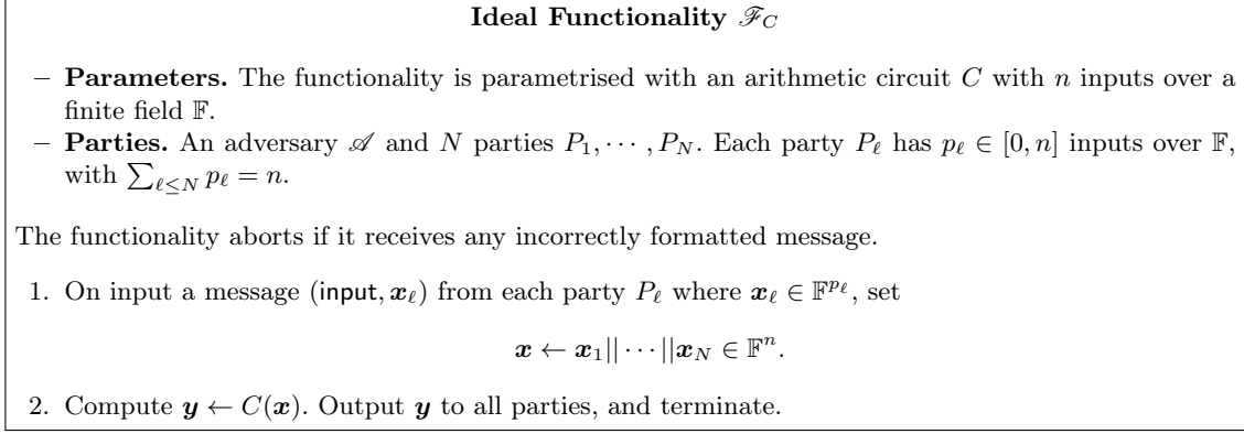
Fig. 2: Ideal functionality \mathcal{F}_C for securely evaluating an arithmetic circuit C among N parties.
