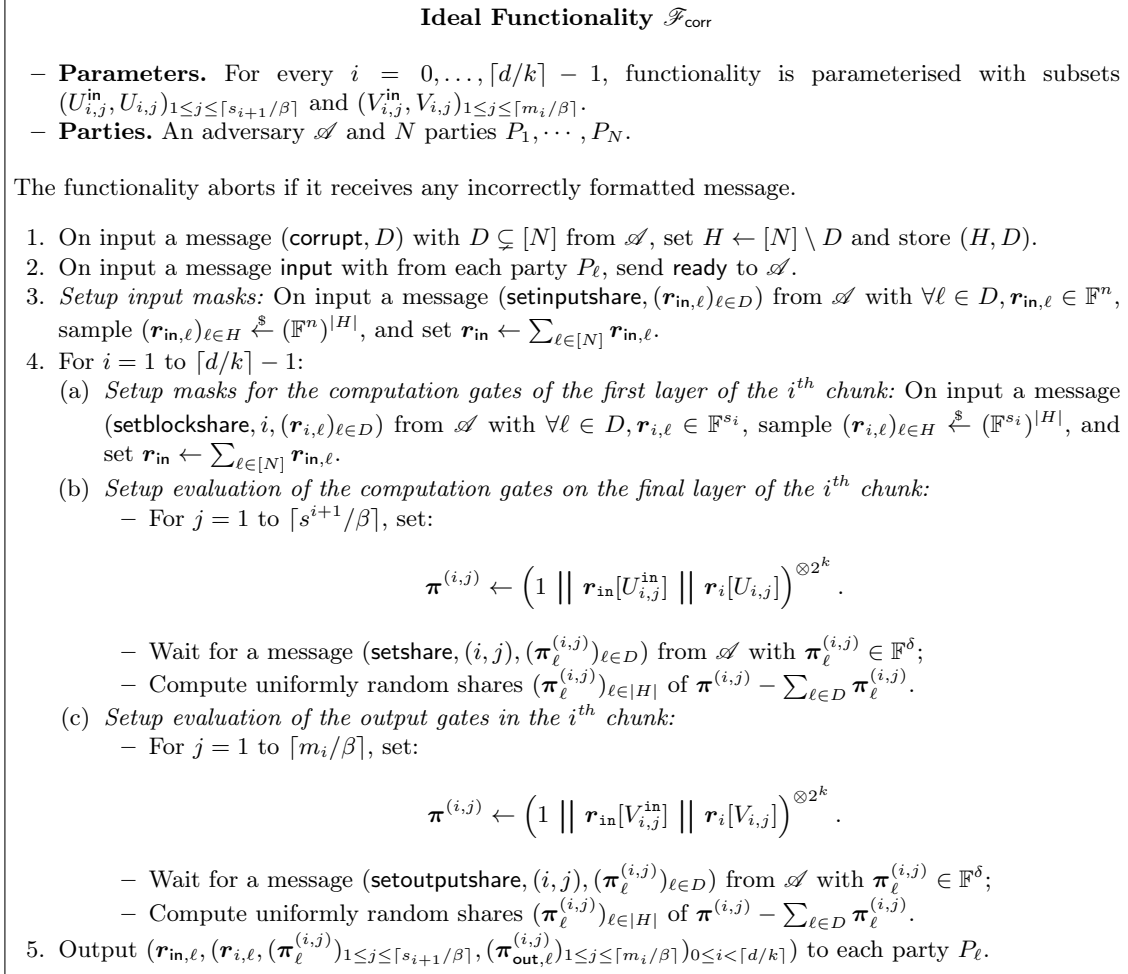
Fig. 3: Ideal corruptible functionality \mathcal{F}_{\text{corr}} to deal out correlated randomness to the parties.
