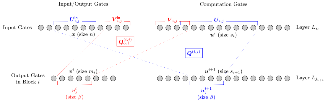
Fig. 4: Decomposition of the i^{\text{th}} Block into low-degree Polynomials.
