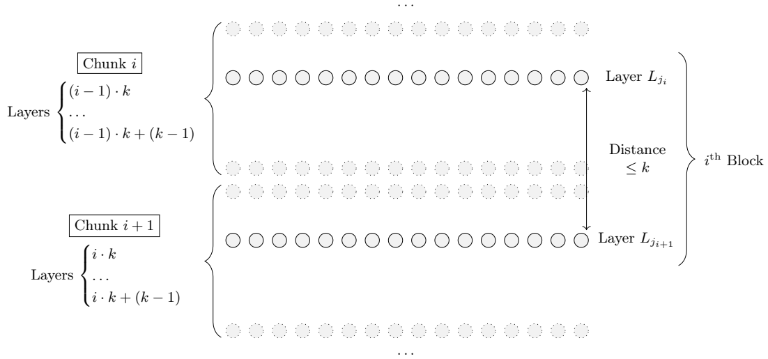
Fig. 1: Block Decomposition of a Circuit.
