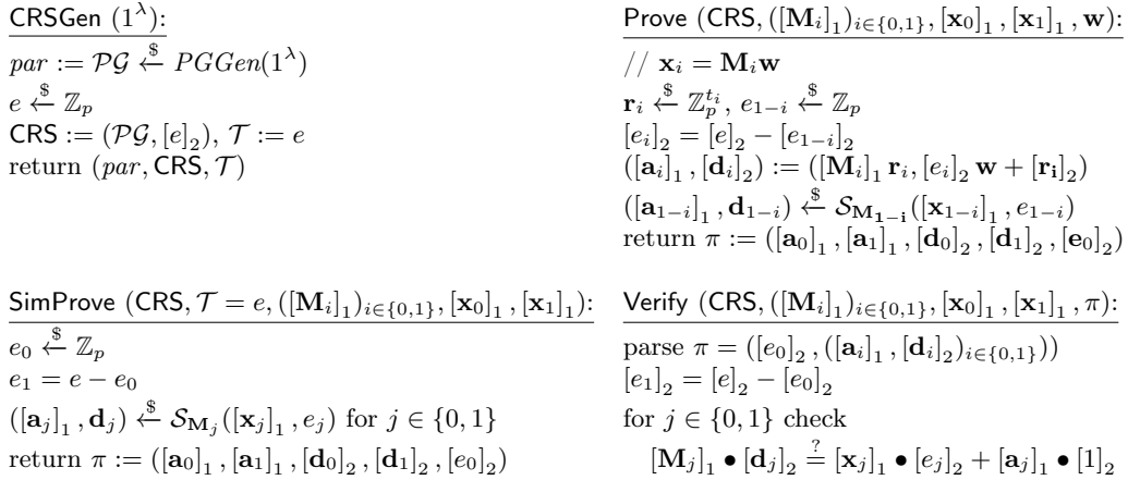
Fig. 6. Compiled protocol \Pi_{\mathbf{M}_0 \vee \mathbf{M}_1}^c \cdot \mathcal{S}_{(\cdot)} denotes the SHVZK-simulator for the respective language.
