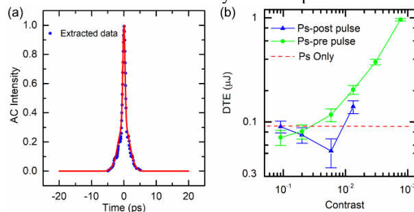
Fig. 1(a) Intensity autocorrelation trace from literature and fitting procedure by combining two components of 800 fs and 4 ps with gaussian approximation. (b) Damage threshold energy (DTE) measurement as function of picosecond contrast measured with double pulse sequences. 'ps-post' signifies the fs component (190 fs) arrives 20 ps ahead of ps component (11ps) whereas 'ps-pre pulse' is the exact opposite.
