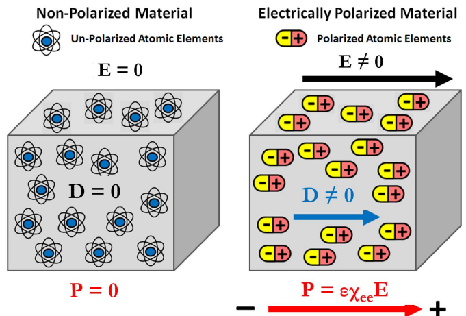
Fig. 16: Example of induced electric dipole moment and electric polarization density ( \mathbf{P} ) in volumetric materials.
