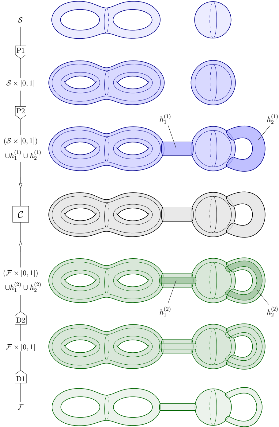
Figure 12: The primal and dual ways of constructing a compression body \mathcal{C} , cf. Section 2.2.
