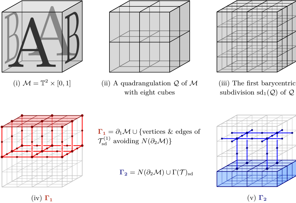
Figure 13: Building a Heegaard splitting of the thickened torus \mathbb{T}^2 \times [0, 1] from a quadrangulation.
