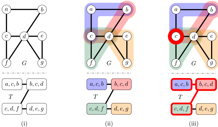
Figure 9: (i) A graph G and a tree decomposition thereof, modeled on a tree T , of width 2. This tree decomposition also happens to be a path decomposition as T is a path. (ii) Illustration of properties 1 and 2 from the definition of a tree decomposition: The union of all bags equals V , and for every arc in E there is a bag containing that arc. (iii) Illustration of property 3: The bags containing a given node (in this case c ) span a connected subtree of T .
