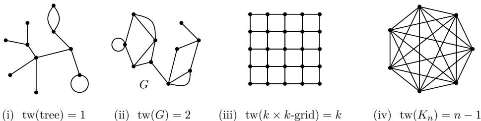
Figure 10: (i) Graphs of treewidth one are precisely the trees (possibly with loops or multiarcs). (ii) A graph of treewidth two. (iii) The k \times k -grid (above k = 5 ) has treewidth and pathwidth equal to k , thus planar graphs can have arbitrary large treewidth. (iv) The complete graph K_n has treewidth n - 1 .
