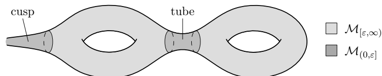
Figure 8: Thick-thin decomposition of a non-compact hyperbolic surface.
