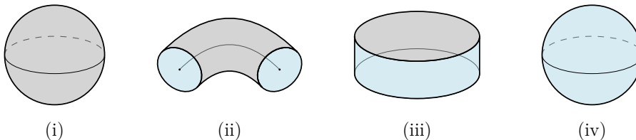
Figure 2: (i) A 0-handle, (ii) a 1-handle, (iii) a 2-handle, and (iv) a 3-handle. The attaching sites are indicated with light blue. For a 1-handle, this is a disjoint union of two disks, for a 2-handle an annulus, and for a 3-handle the entire 2-sphere boundary.
