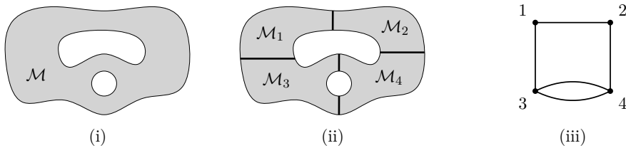
Figure 3: (i) Schematic of a closed 3-manifold \mathcal{M} with nontrivial first homology, (ii) a decomposition \mathcal{D} of \mathcal{M} into four submanifolds, and (iii) the dual graph \Gamma(\mathcal{D}) of \mathcal{D} .
