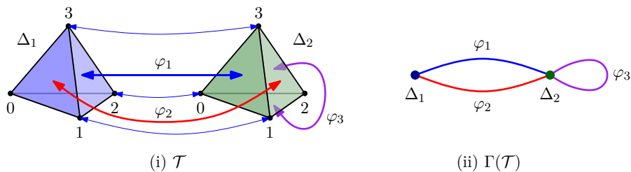
Figure 1: (i) A triangulation \mathcal{T} = \tilde{\Delta}/\Phi with two tetrahedra \tilde{\Delta} = \{\Delta_1, \Delta_2\} and three face gluing maps \Phi = \{\varphi_1, \varphi_2, \varphi_3\} . \varphi_1 is specified to be \Delta_1(123) \xleftrightarrow{\varphi_1} \Delta_2(103) . (ii) The dual graph \Gamma(\mathcal{T}) of \mathcal{T} .
