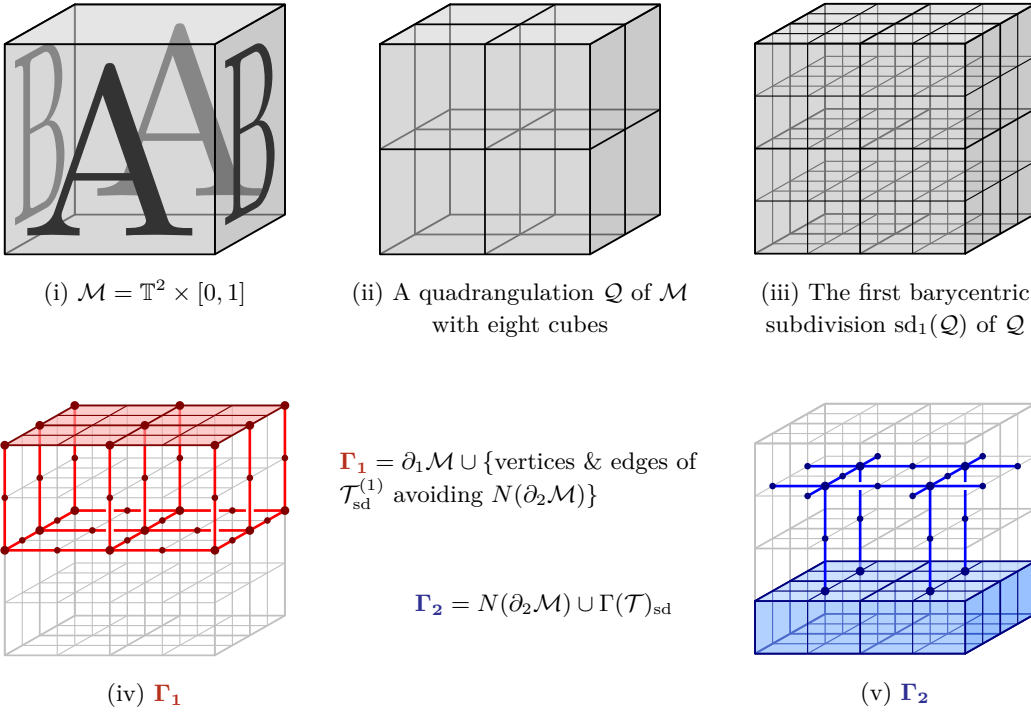
Figure 13: Building a Heegaard splitting of the thickened torus \mathbb{T}^2 \times [0, 1] from a quadrangulation.
