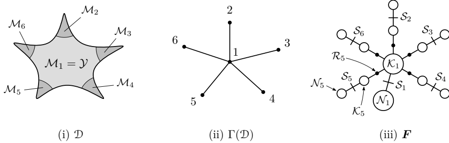
Figure 11: (i) Schematic example of a thick-thin decomposition \mathcal{D} of a hyperbolic 3-manifold \mathcal{M} . (ii) The dual graph \Gamma(\mathcal{D}) of \mathcal{D} with its nodes labeled via the identity map. (iii) The fork complex \mathbf{F} of a generalized Heegaard splitting associated with \mathcal{D} and the given labeling of V(\Gamma(\mathcal{D}))
