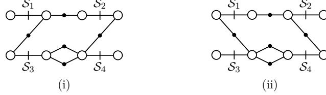
Figure 6: Fork complexes representing the generalized Heegaard splittings shown on Figure 4.
