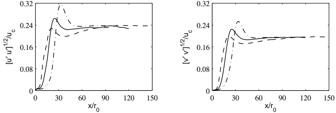
FIG. 5 – Variations along the jet centerline of axial and radial turbulence intensities [u'u']^{1/2}/u_c (left) and [v'v']^{1/2}/u_c (right), for : - - - jetRe1800, — jetRe3600, and - · - jetRe11000.
