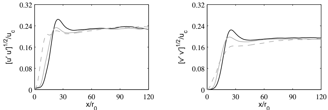
FIG. 6 – Variations along the jet centerline of axial and radial turbulence intensities [u'u']^{1/2}/u_c (left) and [v'v']^{1/2}/u_c (right), for : — jetRe3600, - - - jetRe3600thin, and - · - jetRe3600mode.
