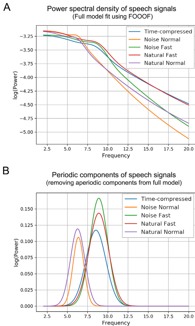
Fig. 2. Power spectra of the acoustic signal for the five conditions. (A) Power spectra of the acoustic signals' envelopes across the five experimental conditions: Natural Normal and Natural Fast correspond to naturally-produced speech at a normal (mean syllable rate 6.76 syllables/s) and fast rate (mean rate 9.15 syll/s), respectively. Time-compressed speech was compressed at the same syllable rate as in the natural fast rate condition (mean syllable rate 9.15 syll/s). Noise Normal and Noise Fast correspond to noise stimuli modulated with the amplitude envelopes of normal rate and fast rate sentences, respectively. The depicted spectra represent parametric model fits of the PSD (Power Spectral Density), that consist of aperiodic and periodic components computed using the FOOOF algorithm (Haller et al., 2018) (B) Periodic components of the full model shown in (A), i.e. after removal of the aperiodic (the so-called 1/f) component of the spectra. The spectral power peaks in the speech stimuli for each condition occur at frequencies that match the corresponding mean syllable rates calculated using the Praat software (see Supplementary Table S1 and Supplementary Fig. S1 for details).
