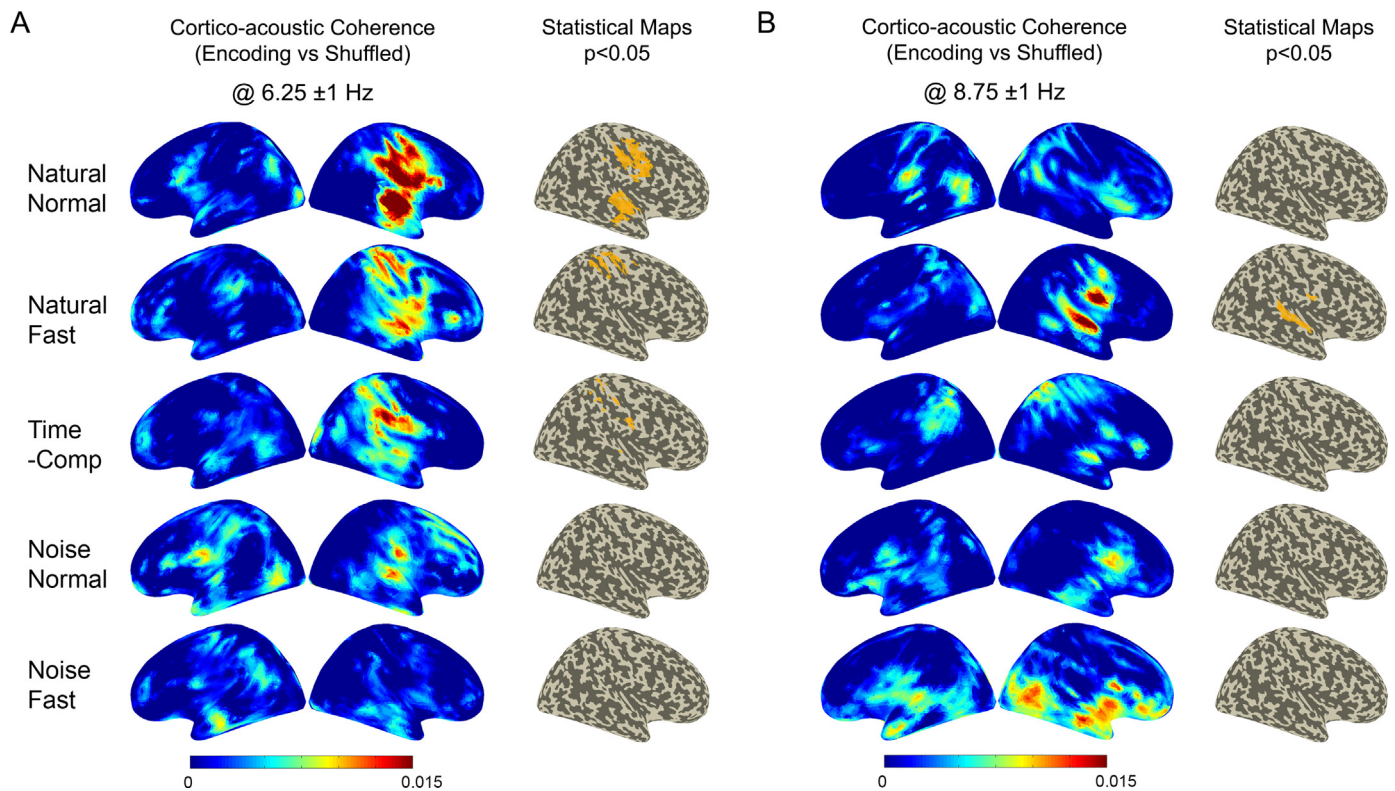
Fig. 3. Cortical tracking of speech at (A) 6.25 ( \pm 1 Hz) and (B) 8.75 ( \pm 1 Hz) matching the normal and fast speech rates respectively. Coherence maps between signal's amplitude envelope and neural oscillations in the active period (i.e. during stimulus presentation), as compared to surrogate data, together with statistical maps in the right hemisphere (corrected, \alpha = 0.05 ; results were not significant in the left hemisphere) presented for the five conditions. Natural Normal = naturally-produced normal rate speech; Natural Fast = naturally-produced fast rate speech; Time-Comp = artificially accelerated speech from normal rate sentences at the same rate as natural fast speech; Noise Normal = amplitude-modulated noise with the envelope of normal rate sentences; Noise Fast = amplitude-modulated noise with the envelope of natural fast rate sentences.
