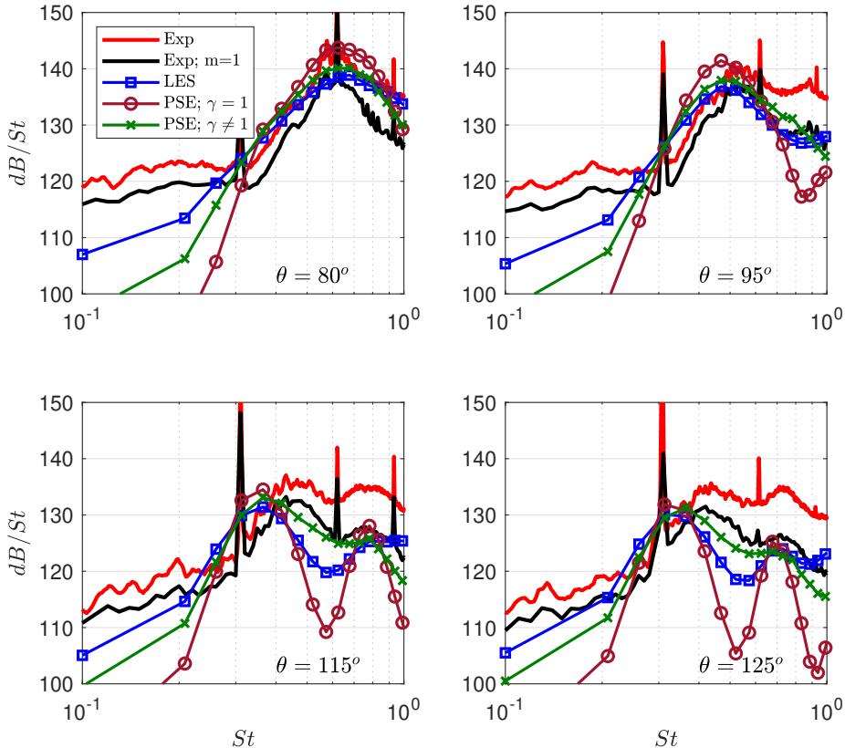
Figure 12: Comparison of acoustic spectra for azimuthal mode m = 1 .
