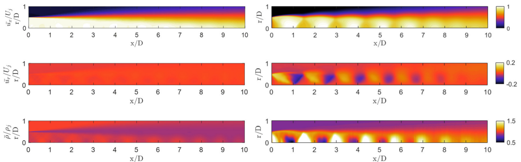
Figure 2: LES (left) and PIV (right) x - r contour mean fields for ideally-expanded and shock-containing jets respectively; streamwise velocity (top), radial velocity (centre) and density (bottom). Flow quantities are normalised by the ideally-expanded condition.
