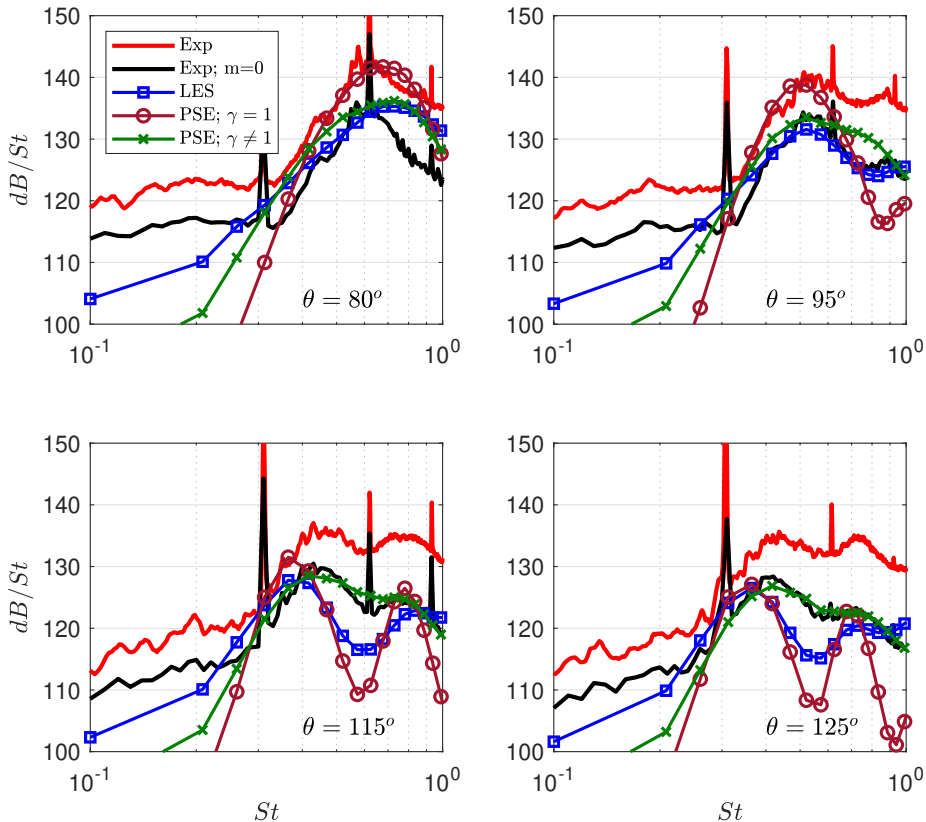
Figure 11: Comparison of acoustic spectra for azimuthal mode m = 0 .
