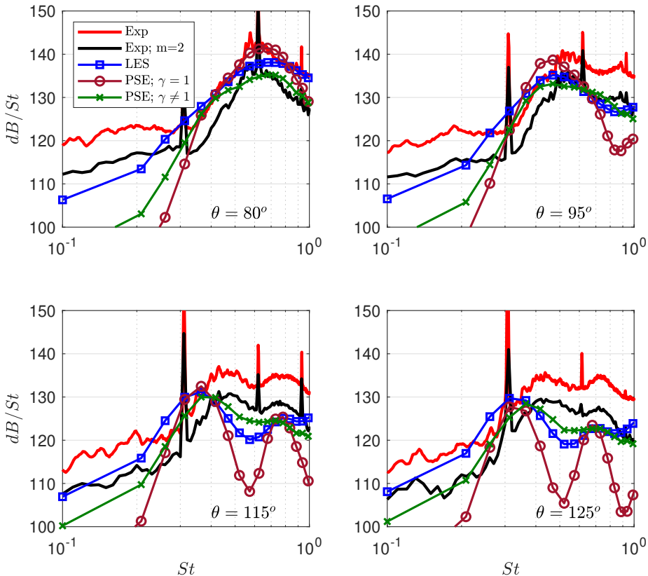
Figure 13: Comparison of acoustic spectra for azimuthal mode m = 2 .
