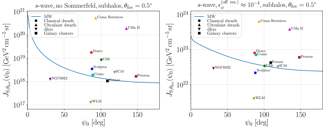
Figure 3: Comparison between J -factors of the various targets in this work and the expected foreground from DM annihilation in the Milky Way halo.
