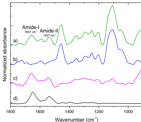
Figure 3. ATR-FTIR absorption spectra ( 1800\text{-}900\text{ cm}^{-1} ) of a) Ge-1-BSA (green) and b) Ge-1-control (blue). Spectrum c) (magenta) is a subtraction of spectrum b to a. Spectrum d) corresponds to native free BSA (black). Spectra a) and b) were normalized with respect to the intensity at 1459\text{ cm}^{-1} and spectra c) and d) were normalized with respect to the intensity of the amide-I band.
