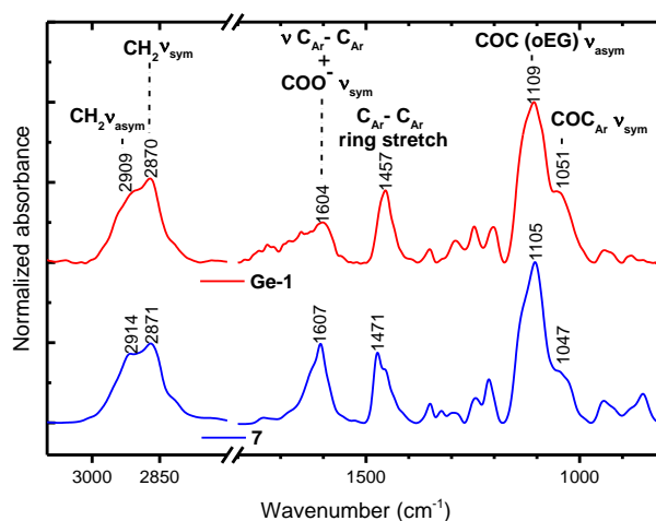
Figure 2. ATR-FTIR absorption spectra (3100-2700 cm -1 and 1800-800 cm -1 ) of modified surface Ge-1 (red) and calix[4]arene 7 (blue). All spectra were normalized with respect to the intensity at 1459 cm -1 .
