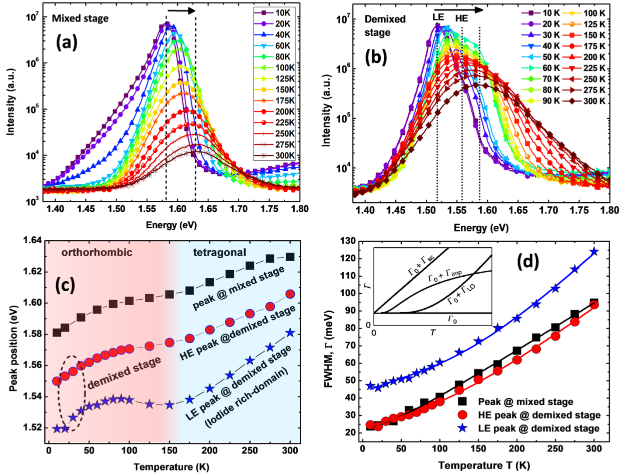
Figure 5: Temperature dependent PL emission characteristics of triple-cation mixed-halide (MA_{0.17}FA_{0.83})_{0.95}Cs_{0.05}Pb(I_{0.83}Br_{0.17})_3 perovskite film in both mixed and demixed (segregated phase) stages. (a) Temperature-dependent PL spectra at low excitation power-density ( P_{exc} = 1 mW/cm 2 ) and (b) PL spectra of demixed stage under excitation with high power-density ( P_{exc} = 840 mW/cm 2 ). (c) A comparison of blue-shift response of emission peaks in both mixed and demixed stages as a function of temperature. (d) The linewidth broadening of PL spectra in both mixed and demixed stages as function of temperature (symbols) along with least square fitting curves (solid lines) to examine the exciton-phonon coupling.
