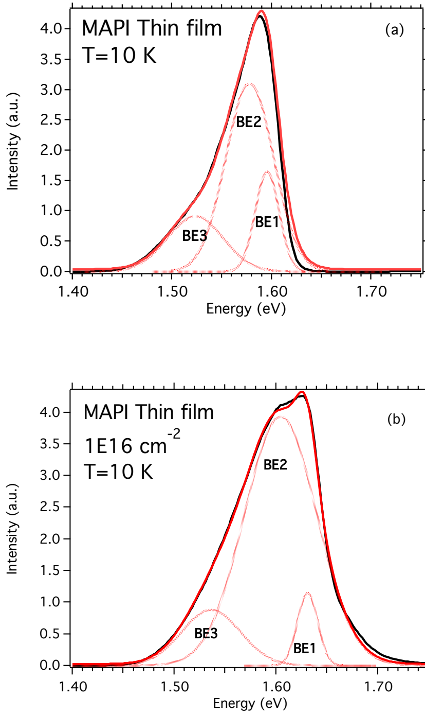
Figure 5: PL spectra from (CH 3 NH 3 )PbI 3 thin films at T=10 K, before (a) and after irradiation with Helium ions at 30 keV 1E16 cm -2 (b). A decomposition of the spectra in three bound exciton components is shown (BE1, BE2 and BE3), together with the fit to the spectra.
