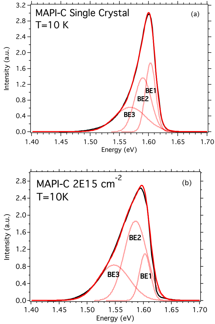
Figure 4: PL spectra from (\text{CH}_3\text{NH}_3)\text{PbI}_3 single crystals at T=10 K, before (a) and after irradiation with Helium ions at 30 \text{ keV } 2\text{E}15 \text{ cm}^{-2} (b). A decomposition of the spectra in three bound exciton components is shown (BE1, BE2 and BE3), together with the fit to the spectra.
