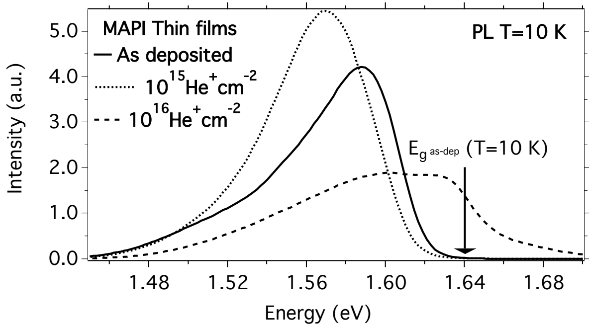
Figure 6: PL spectra from (\text{CH}_3\text{NH}_3)\text{PbI}_3 thin films at T=10 \text{ K} , before and after irradiation with Helium ions at 30 \text{ keV} 1\text{E}15 \text{ cm}^{-2} and 1\text{E}16 \text{ cm}^{-2} .
