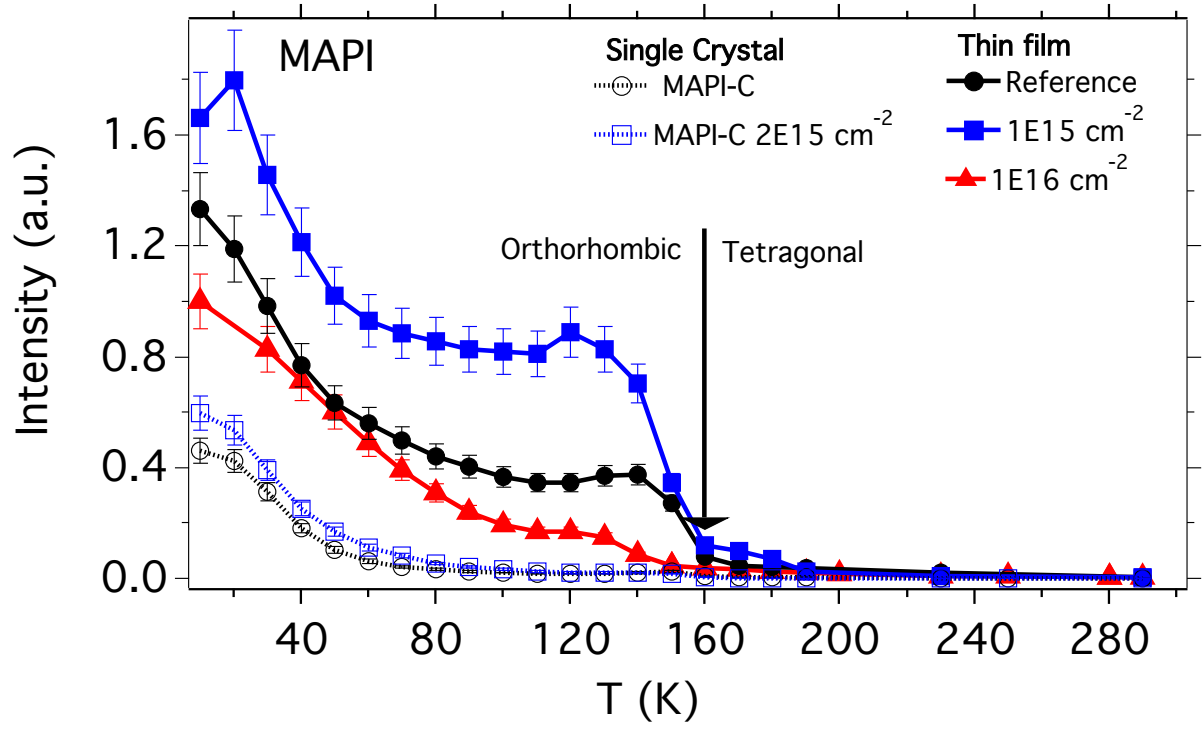
Figure 8: Temperature dependence of the PL integrated intensity from (\text{CH}_3\text{NH}_3)\text{PbI}_3 thin films and single crystals, before and after irradiation with Helium ions at 30 keV 1E15 cm -2 and 1E16 cm -2 for thin films and 2E15 cm -2 for the single crystal. The integrated intensity for the reference MAPI thin film was normalized to 1 at T=10 K.
