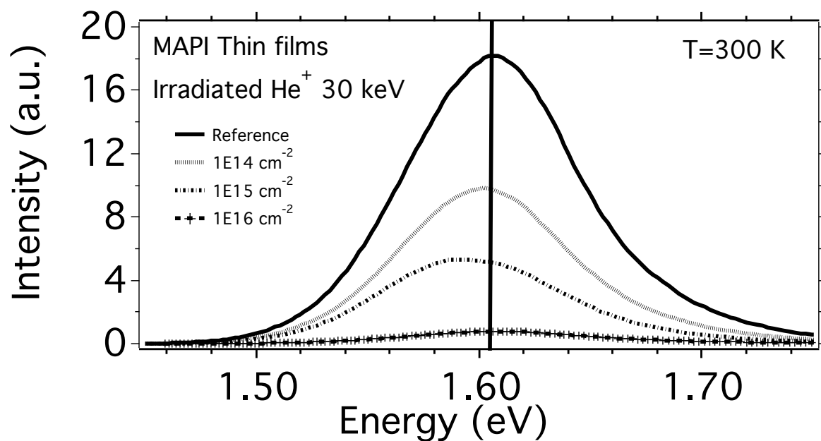
Figure 1 : PL spectra from (\text{CH}_3\text{NH}_3)\text{PbI}_3 polycrystalline thin films at room temperature after irradiation with Helium ions at 30 keV and different fluences between 10^{14} \text{ cm}^{-2} and 10^{16} \text{ cm}^{-2} .
