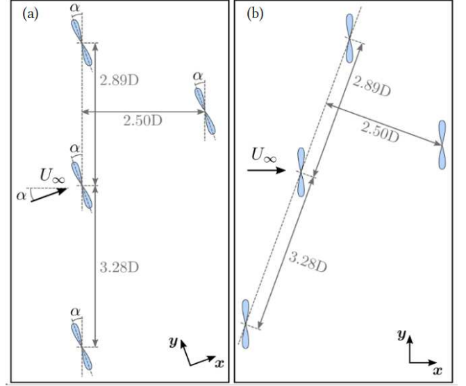
Fig. 3: Four tidal turbine array configuration based on the NEPHTHYD project configuration and reproduced from information given in [1]. (a) Configuration with an incoming flow yawed with an angle \alpha . (b) Similar representation but for which the flow is represented horizontally.
