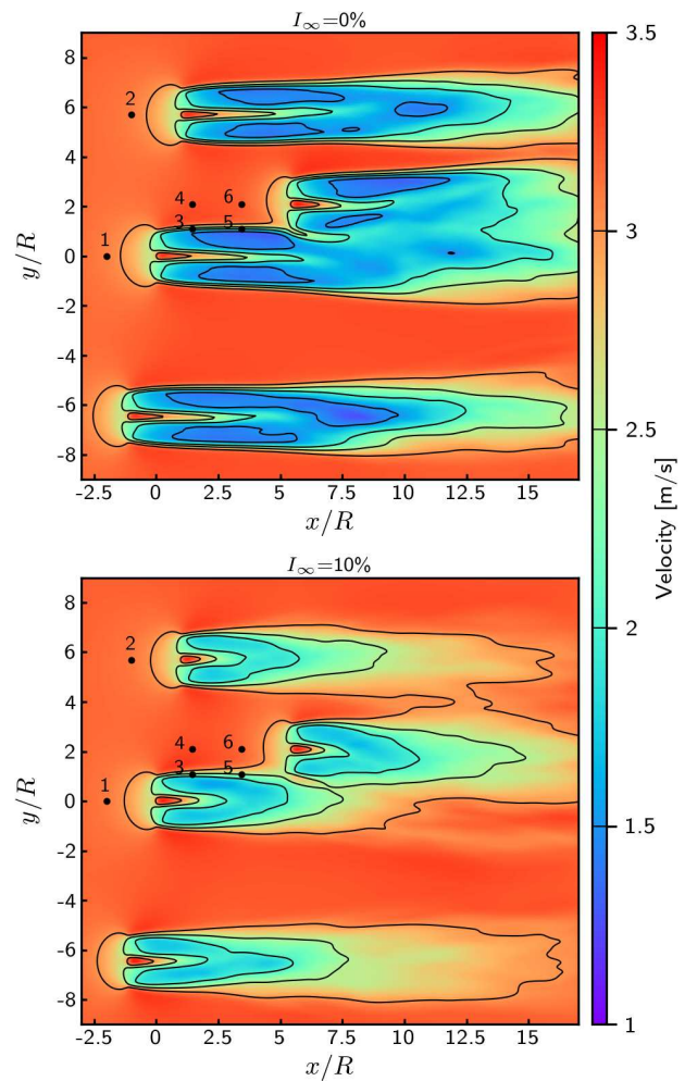
Fig. 4: Time-averaged velocity wake maps, I_\infty=0\% and I_\infty=10\% .
