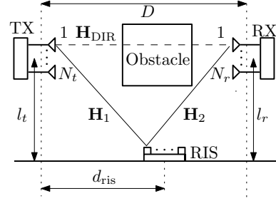
Fig. 1. Aerial view of the considered communication system.
