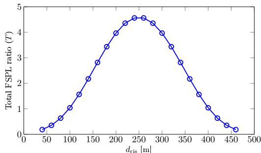
Fig. 4. The total FSPL ratio ( T ) for the case l_t = l_r = 50 m.
