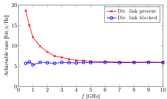
Fig. 9. Average achievable rate versus frequency f . The parameter setup is the same as for Fig. 2.
