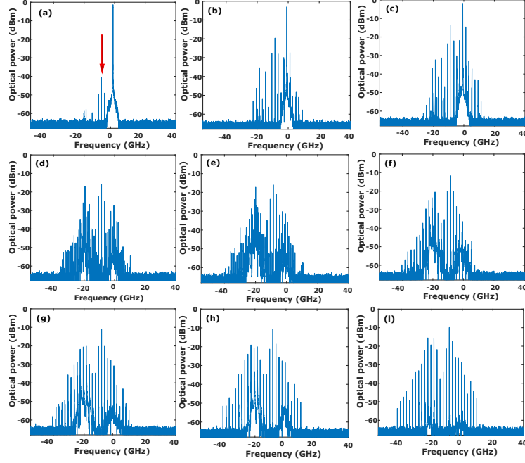
Fig. 8. Scenario C: Optical spectra of two polarization OFC dynamics for fixed comb spacing to \Omega = 2 GHz, and detuning \Delta\nu = -6.5 GHz. (a), (b) and (c), unlocked dynamics at P_{inj} = 0.3 \mu\text{W} , P_{inj} = 80 \mu\text{W} and P_{inj} = 216 \mu\text{W} , respectively, (d) incomplete PS at P_{inj} = 224 \mu\text{W} , (e) complex harmonic comb in both polarization modes at P_{inj} = 408 \mu\text{W} , (f) and (g) complex comb in both polarization modes at P_{inj} = 520 \mu\text{W} and P_{inj} = 576 \mu\text{W} , respectively, (h) and (i) comb in both polarization modes P_{inj} = 600 \mu\text{W} and P_{inj} = 640 \mu\text{W} , respectively. The red arrow in optical spectrum of (a) indicates the position of the central injected comb line.
