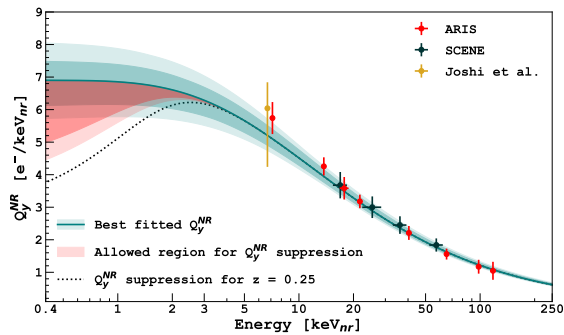
FIG. 11. Allowed region (red) for low energy Q_y^{NR} suppression tested on the AmC dataset, and best fitted Q_y^{NR} (blue), using the Ziegler et al. screening function. Dark (light) shaded area corresponds to 1\sigma ( 2\sigma ) uncertainty. The dashed line represents the Q_y^{NR} suppression tested in [36] assuming eq. 16 with z=0.25 .
