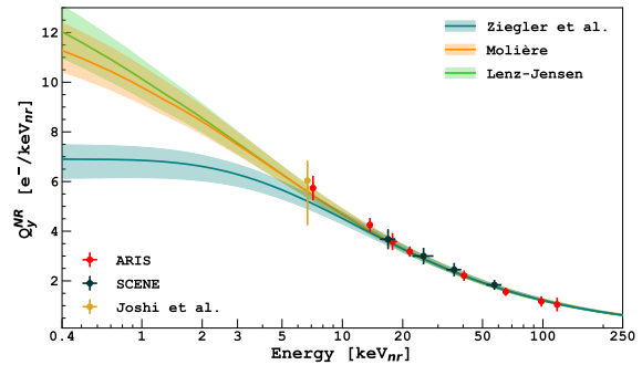
FIG. 10. Fit of DarkSide-50 AmBe and AmC data, and ARIS and SCENE datasets using Ziegler et al. (eq. 13) [37], Molière [43], and Lenz-Jensen [44, 45] screening functions. The model bands correspond to 1\sigma uncertainty.
