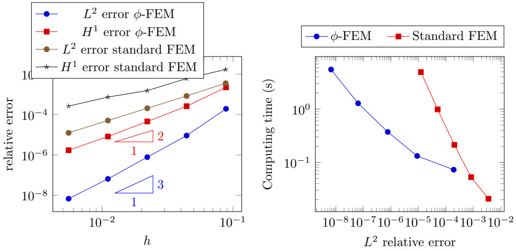
Figure 7: Test case with mixed boundary conditions, results on meshes as on Fig. 6. Left: L^2 and H^1 relative errors under the mesh refinement. Right: computing time vs. the L^2 relative error.
