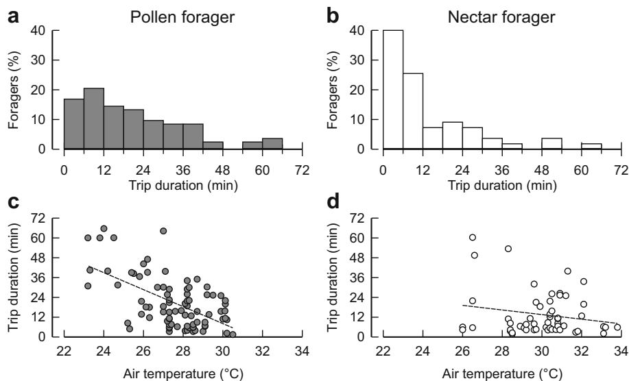
Figure 1. Association between foraging trip duration and air temperature in foragers of Melipona subnitida . Frequency distribution of foraging trip durations in a pollen foragers and b nectar foragers. Scatterplots showing the association between foraging trip duration and air temperature in c pollen foragers and d nectar foragers. Grey bars and circles: pollen foragers ( n = 83 ); white bars and circles: nectar foragers ( n = 55 ). Dashed lines: linear regression ( c , R^2 adj = 0.329, P < 0.001 ; d , R^2 adj = 0.018, P = 0.164 ).
