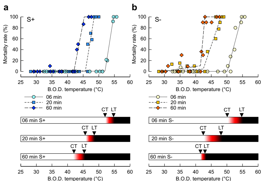
Figure 2. Plasticity of upper thermal limits in foragers of Melipona subnitida . Given are mortality rates of forager groups maintained in mesh cages within B.O.D incubators at the given temperatures for 6 min (circles), 20 min (squares), or 60 min (diamonds). Each symbol represents one experimental group comprising between 10 and 15 individuals. Prior to heat exposure, experimental groups either received liquid food (a, treatment S+) or remained unfed (b, treatment S-). Black dashed lines indicate Three-Segment Linear Regressions used to estimate critical temperatures (CT) and lethal temperatures (LT) of the experimental treatments.
