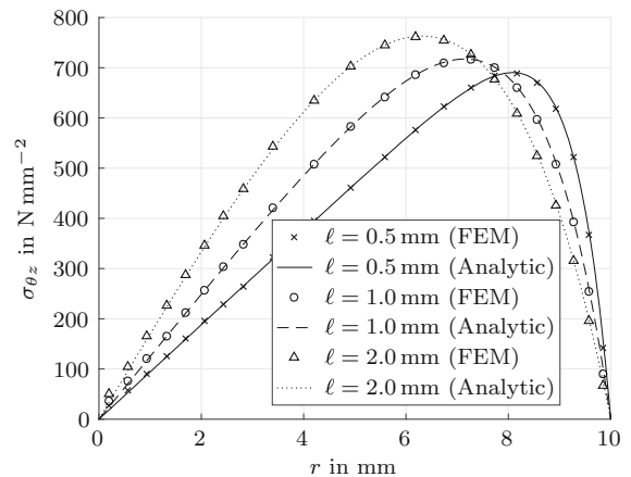
Fig. 11 Comparison between the analytic and numerical predictions for the shear stress distribution in torsion for the stress gradient continuum endowed with three different intrinsic length scales ( E = 210,000 \text{ N/mm}^2 , \nu = 0.3 )
