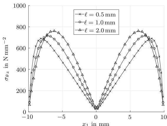
Fig. 9 Shear stress distribution predicted by finite element simulations of the torsion problem depicted in Fig. 8 ( E = 210,000 N/mm 2 , \nu = 0.3 )
