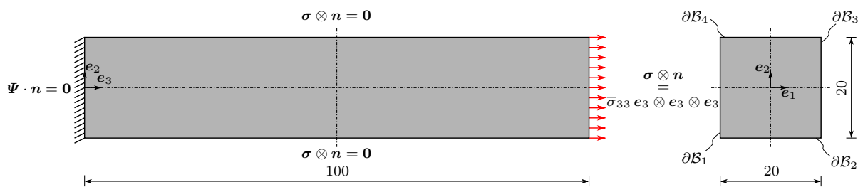
Fig. 5 Geometric dimensions (in mm) and boundary conditions of the rectangular bar under tension
