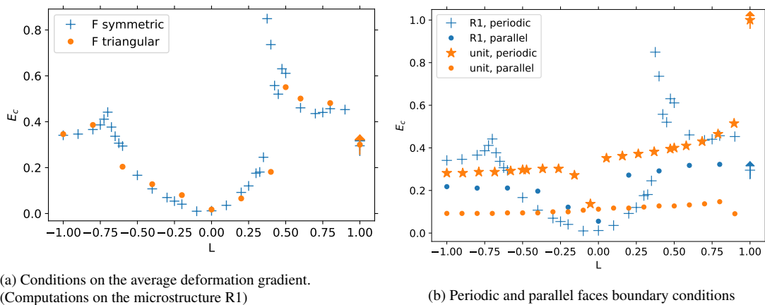
Fig. 19: Influence of boundary conditions on the response of the cell. All computations at triaxiality T = 1 .
