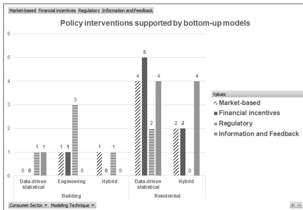
Figure 7. Distribution policy instruments supported by bottom-up models.
