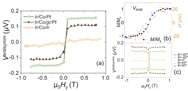
FIG. 3. Thermo-spin voltage in epitaxial hybrid gr/HM and HM stacks. (a) Thermo-spin voltage in Ir/Co/Ir, Ir/Co/Pt, and Ir/Co/gr/Pt. The observed thermo-spin voltage in the sample with the Ir capping layer (yellow) is significantly smaller than that with Pt, and it is mainly due to the anomalous Nernst effect in Co. A reduction in the voltage at saturation field is observed when gr is introduced into the stack. (b) Close-up view on the anomalous Nernst effect voltage in the Ir/Co/Ir sample and its magnetization measured by vibrating sample magnetometry. (c) Angular dependence on the thermo-spin voltage in the Ir/Co/Pt sample. The angle \theta represents the relative angle between the measured voltage (x direction) and the applied magnetic field (xy plane).
