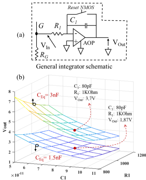
Fig.13. (a). Basic integrator schematic (b). 3D plot of the integrator output V_{Out} under different variation. [16], with R_I \gg R_G & C_I \gg C_{Stray}
