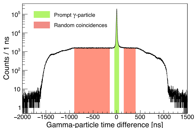
FIG. 2. \gamma -particle coincidence spectrum. The gate used to select the prompt coincidences is marked in green (light gray), while the two regions considered for the random-coincidence subtraction are marked in red (dark gray).
