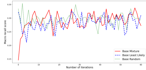
(b) Recall
