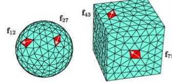
FIG. 10 Collage of selected computational methods. Schematics of basis functions, along with selected results, for spectral (Bimonte et al., 2017; Krüger et al., 2012; McCauley et al., 2012; Messina and Antezza, 2011b; Messina et al., 2017b), finite-difference (Jin et al., 2019; Rodriguez et al., 2011; Werner et al., 2013), volume integral (Polimeridis et al., 2015), and surface integral (Reid et al., 2013b; Rodriguez et al., 2013a,b) methods.
