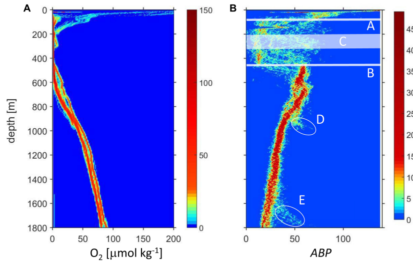
FIGURE 2 | Depth profiles of oxygen (A) and ABP (B). The color indicates the number of data in a bin, for oxygen ( 4\text{ m} \times 0.5\ \mu\text{mol kg}^{-1} ), for ABP ( 4\text{ m} \times 0.7 ). In (B) are indicated: (A) Approximate depth of the upper oxycline. (B) Depth of the lower oxycline ( lOx ). (C) The depth of the intermediate oxygen maximum ( iO_2 ) only encountered on some stations; ellipses (D,E): data from two stations on the shelf break.
