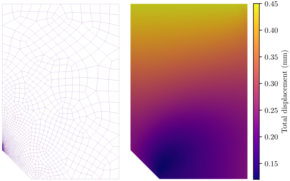
Figure 15: The mesh of the rhombus hole specimen for the angle \gamma = 90^\circ , and the total displacements of the mesh at the end of the test, measured by the norm of the displacements at each node.
