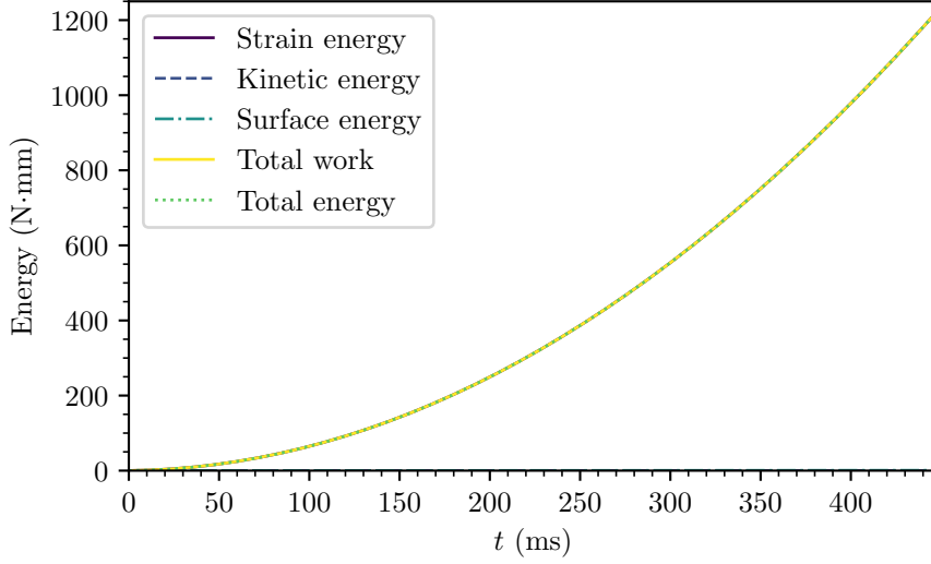
Figure 17: The energies of the rhombus hole simulation.
