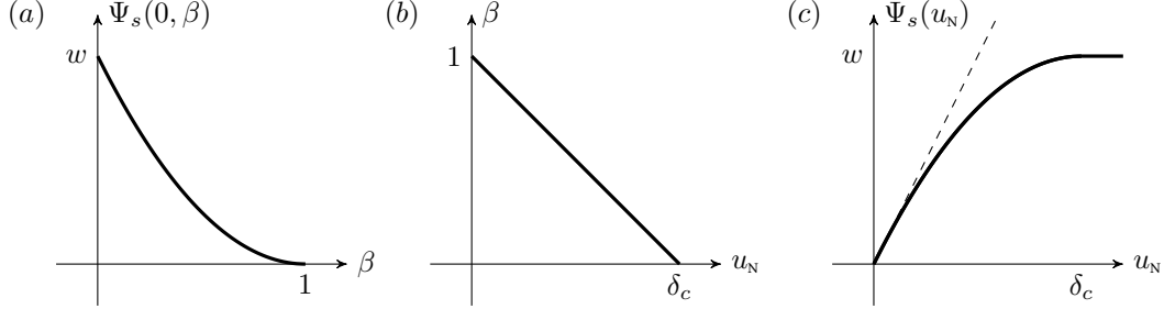
Figure 1: (a) The shape of the surface potential \Psi_s with respect to \beta . (b) The consequent linear evolution of \beta with u_N . (c) The shape of the surface potential \Psi_s with respect to u_N , where the initial slope is equivalent to the value of \sigma_c , and the final value is w .
