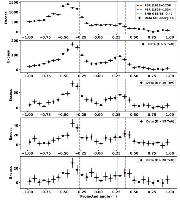
Fig. 2. Distribution of VHE \gamma -ray excess along axis of the cyan dashed rectangle indicated in Fig. 1 that encompasses both HESS J1825–137 (broad peak on the left) and HESS J1826–130 (shallower peak on the right, becoming apparent only at high energies) above 0.4 TeV and at E > 5 TeV, 10 TeV, 15 TeV, and 20 TeV. Vertical lines show the position of PSR J1826–1256 (red), PSR J1826–1334 (blue) and SNR G18.45–0.42 (red).
