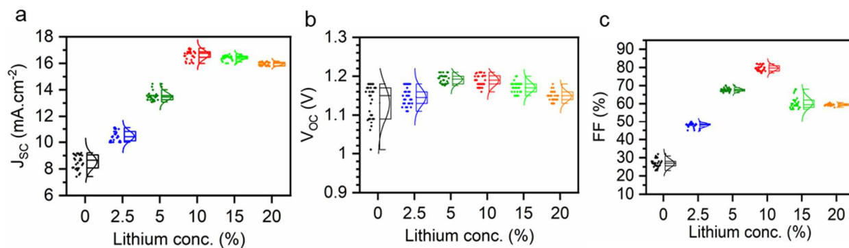
Figure S13. Solar cell performance of 2D perovskite devices. a-c) Statistics of the photovoltaic parameters of BA 2 MA 3 Pb 4 I 13 2D perovskite solar cells fabricated on top of NiOx HTL with different doping concentration of Li.
