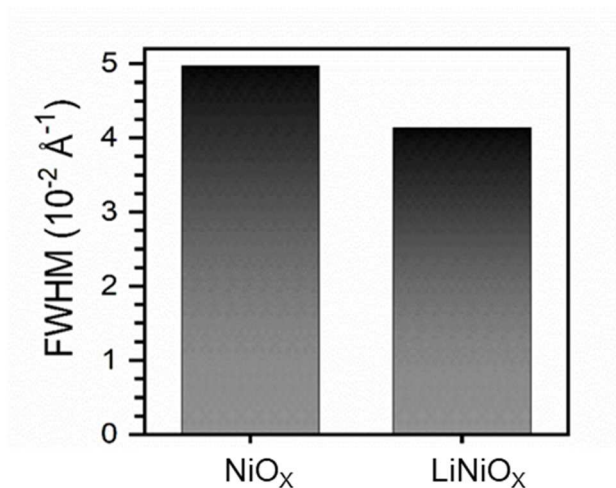
Figure S10. Crystallinity of the 2D perovskite film extracted from the GIWAXS measurements. Full width at half maximum (FWHM) evaluated from the angular integration of the GIWAXS patterns of BA 2 MA 3 Pb 4 I 10 films fabricated on top of the pristine NiO x and Li-doped NiO x .
