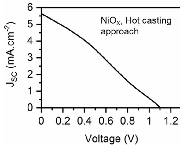
Figure S14. Solar cell characteristics of Hot casting approach. Current-voltage characteristics of the of BA 2 MA 3 Pb 4 I 13 2D perovskite solar cell fabricated on pristine NiO x using hot casting approach.
