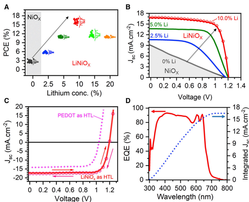
Figure 3. Photovoltaic characteristics of the 2D perovskite solar cell with the \text{NiO}_x HTL
