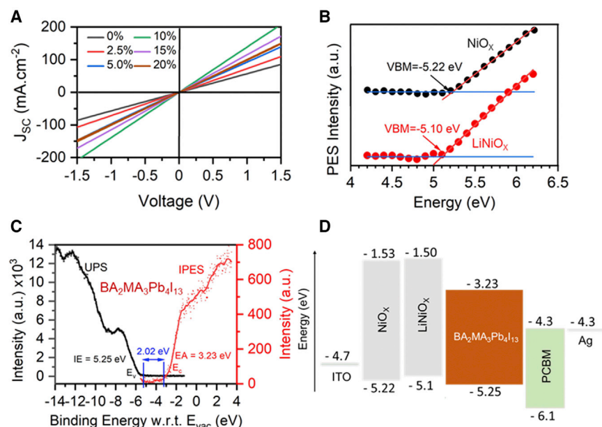
Figure 4. Electronic characteristics of 2D perovskite solar cell with pristine and Li-doped \text{NiO}_x
