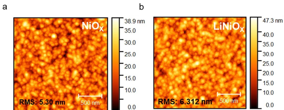
Figure S3. Morphology of the nickel oxide hole transport layer. a) Morphology of the pristine \text{NiO}_x and Li-doped \text{NiO}_x with the extracted root-mean-square roughness obtained by atomic force microscopy.
