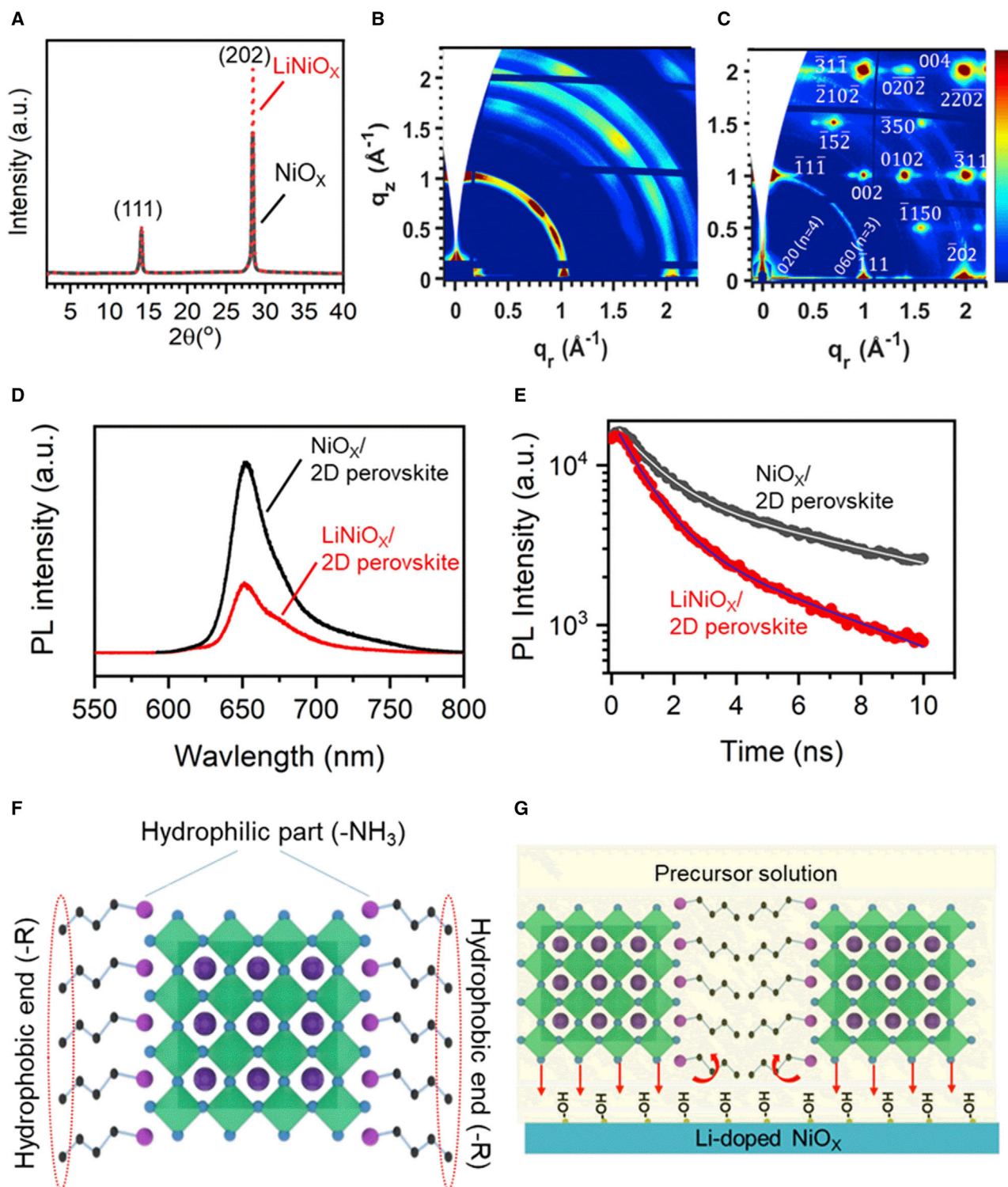
Figure 2. Orientation and interfacial characteristics of 2D perovskite on NiOx surfaces
