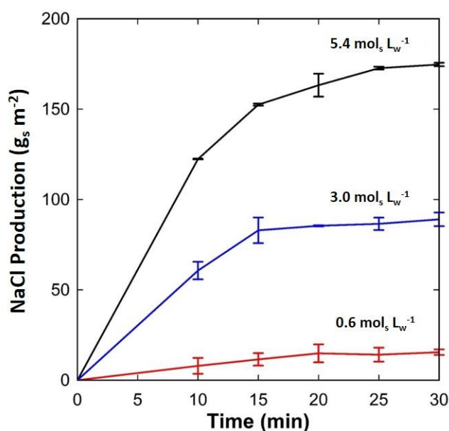
279 Fig. 6. NaCl production as a function of pervaporation time for a porous membrane tube thickness 280 of 2.5 mm for various NaCl feed concentration (0.6, 3.0 and 5.4 mol s L w -1 ). The membranes were 281 oven dried at 60 °C for 8 h and RH = 67.3%. 282
