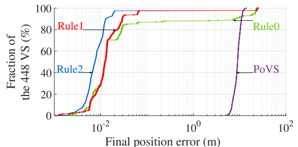
Fig. 3: Cumulative distribution of position errors.
