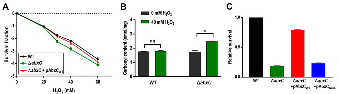
Figure 3. Effects of abxC mutation on H 2 O 2 resistance. (A) Survival of \Delta abxC exposed to H 2 O 2 . WT, \Delta abxC , and \Delta abxC harboring pAbxC WT that encodes the wild-type AbxC were treated with H 2 O 2 at the indicated concentrations for 1 h. The survival fraction was calculated by dividing the CFU of H 2 O 2 -treated cells by the CFU of non-treated cells. Values are means and standard deviations of two independent experiments conducted in duplicate. (B) Protein carbonylation of \Delta abxC in response to H 2 O 2 . After treatment of 40 mM H 2 O 2 for 1 h, the carbonylated protein contents of WT and \Delta abxC were measured by the 2,4-dinitrophenylhydrazine (DNPH) assay. Data represent the means \pm standard deviations of three independent experiments. Comparisons between two groups were performed by Student's t -test (GraphPad Prism 7.04). A p -value of less than 0.01 is considered statically significant (ns; not significant, *; p < 0.01). (C) Complementation of \Delta abxC . WT, \Delta abxC , and \Delta abxC harboring the pAbxC WT and pAbxC C36S plasmids, which produce the wild-type AbxC and its C36S mutant proteins, respectively, were treated with 40 mM H 2 O 2 for 1 h. Survival abilities of \Delta abxC mutants were expressed relative to WT survival (arbitrarily set at 1), i.e., the CFU of mutants were normalized to the CFU of WT. Data represent the means \pm standard deviations of three independent experiments.
